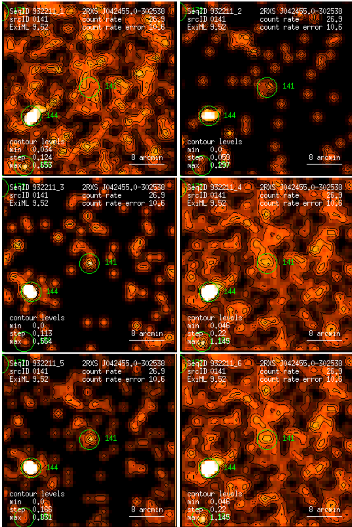
Figure 141: RASS 932211: detection 0141: band rate images, Gaussian filter: (1) PSPC channels 11 – 41, (2) 52 – 90, (3) 91 – 201, (4) 11 – 235, (5) 52 – 201, (6) 11 – 201. Broad band rates in counts/ks. Band rate contour levels in counts/ks/arcmin 2 .
