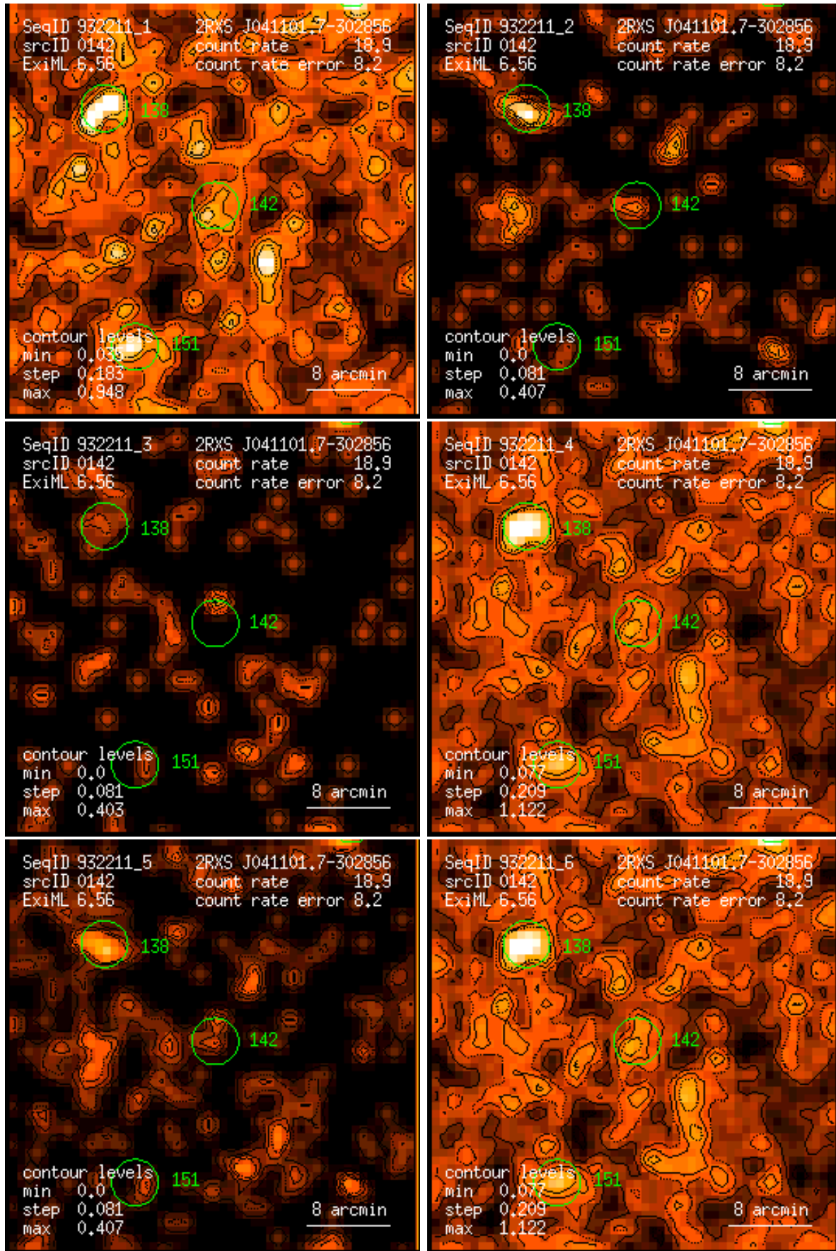
Figure 142: RASS 932211: detection 0142: band rate images, Gaussian filter: (1) PSPC channels 11 – 41, (2) 52 – 90, (3) 91 – 201, (4) 11 – 235, (5) 52 – 201, (6) 11 – 201. Broad band rates in counts/ks. Band rate contour levels in counts/ks/arcmin 2 .
