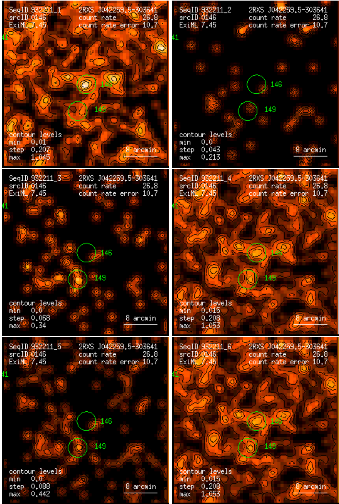
Figure 146: RASS 932211: detection 0146: band rate images, Gaussian filter: (1) PSPC channels 11 – 41, (2) 52 – 90, (3) 91 – 201, (4) 11 – 235, (5) 52 – 201, (6) 11 – 201. Broad band rates in counts/ks. Band rate contour levels in counts/ks/arcmin 2 .
