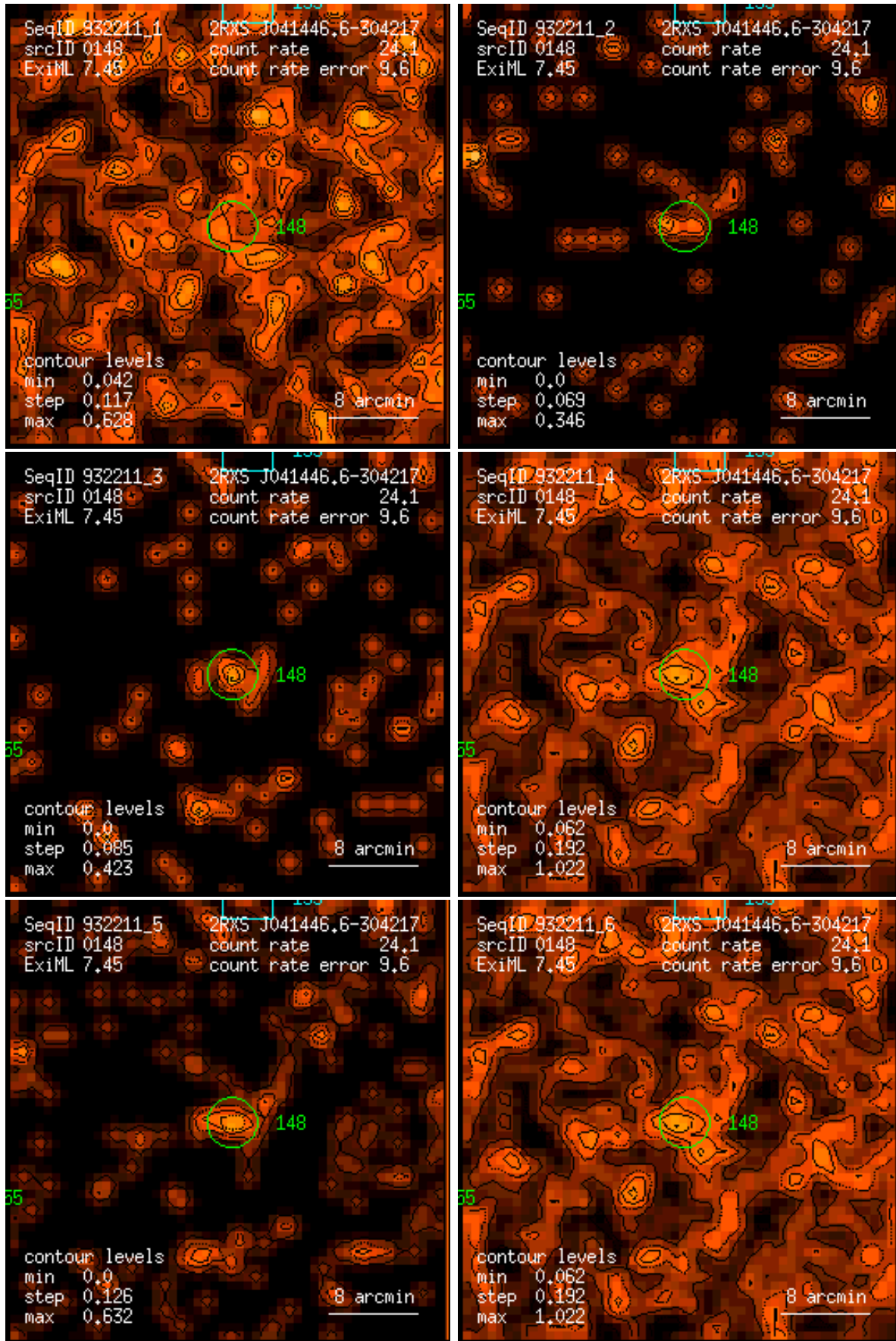
Figure 148: RASS 932211: detection 0148: band rate images, Gaussian filter: (1) PSPC channels 11 – 41, (2) 52 – 90, (3) 91 – 201, (4) 11 – 235, (5) 52 – 201, (6) 11 – 201. Broad band rates in counts/ks. Band rate contour levels in counts/ks/arcmin 2 .
