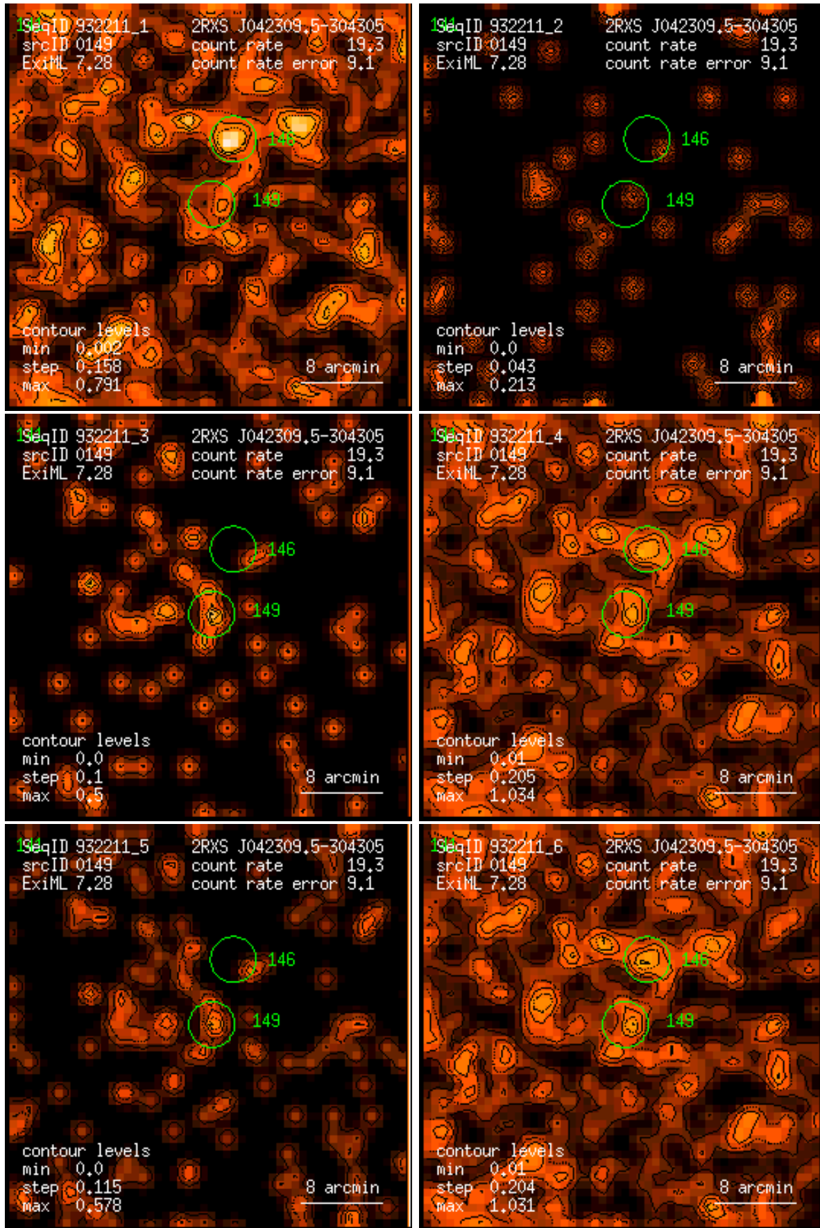
Figure 149: RASS 932211: detection 0149: band rate images, Gaussian filter: (1) PSPC channels 11 – 41, (2) 52 – 90, (3) 91 – 201, (4) 11 – 235, (5) 52 – 201, (6) 11 – 201. Broad band rates in counts/ks. Band rate contour levels in counts/ks/arcmin 2 .
