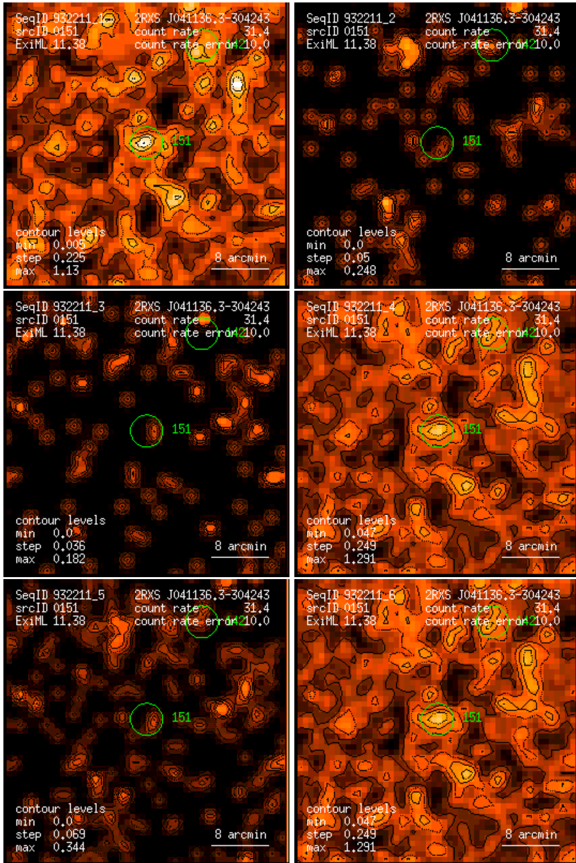
Figure 151: RASS 932211: detection 0151: band rate images, Gaussian filter: (1) PSPC channels 11 – 41, (2) 52 – 90, (3) 91 – 201, (4) 11 – 235, (5) 52 – 201, (6) 11 – 201. Broad band rates in counts/ks. Band rate contour levels in counts/ks/arcmin 2 .
