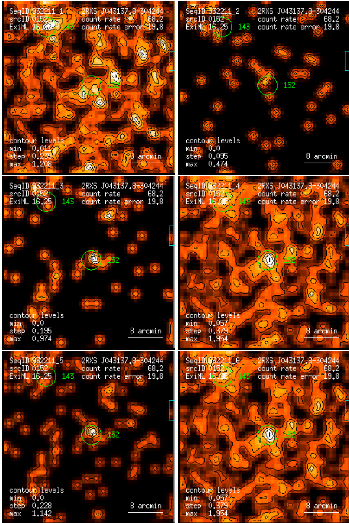
Figure 152: RASS 932211: detection 0152: band rate images, Gaussian filter: (1) PSPC channels 11 – 41, (2) 52 – 90, (3) 91 – 201, (4) 11 – 235, (5) 52 – 201, (6) 11 – 201. Broad band rates in counts/ks. Band rate contour levels in counts/ks/arcmin 2 .
