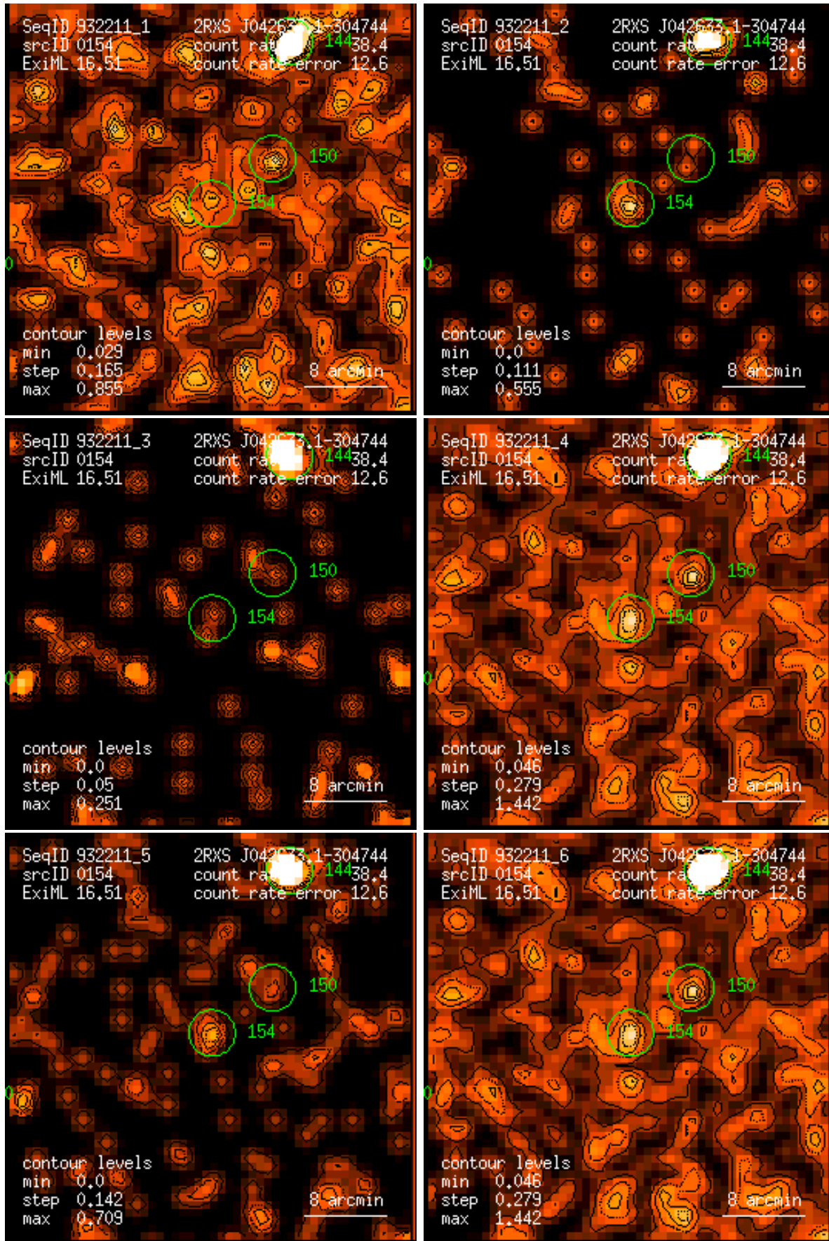
Figure 154: RASS 932211: detection 0154: band rate images, Gaussian filter: (1) PSPC channels 11 – 41, (2) 52 – 90, (3) 91 – 201, (4) 11 – 235, (5) 52 – 201, (6) 11 – 201. Broad band rates in counts/ks. Band rate contour levels in counts/ks/arcmin 2 .
