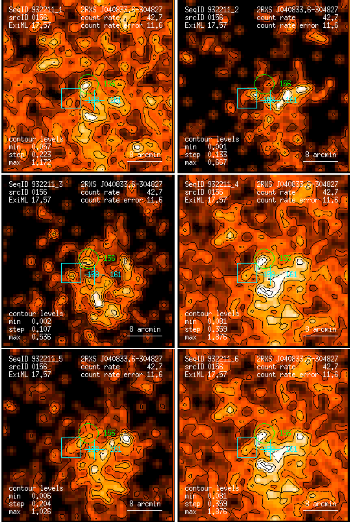
Figure 156: RASS 932211: detection 0156: band rate images, Gaussian filter: (1) PSPC channels 11 – 41, (2) 52 – 90, (3) 91 – 201, (4) 11 – 235, (5) 52 – 201, (6) 11 – 201. Broad band rates in counts/ks. Band rate contour levels in counts/ks/arcmin 2 .
