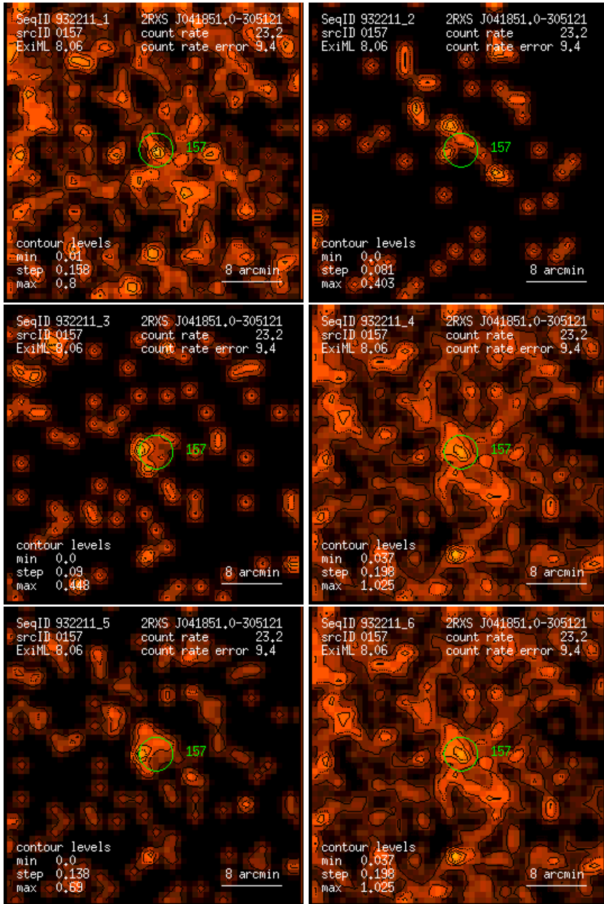
Figure 157: RASS 932211: detection 0157: band rate images, Gaussian filter: (1) PSPC channels 11 – 41, (2) 52 – 90, (3) 91 – 201, (4) 11 – 235, (5) 52 – 201, (6) 11 – 201. Broad band rates in counts/ks. Band rate contour levels in counts/ks/arcmin 2 .
