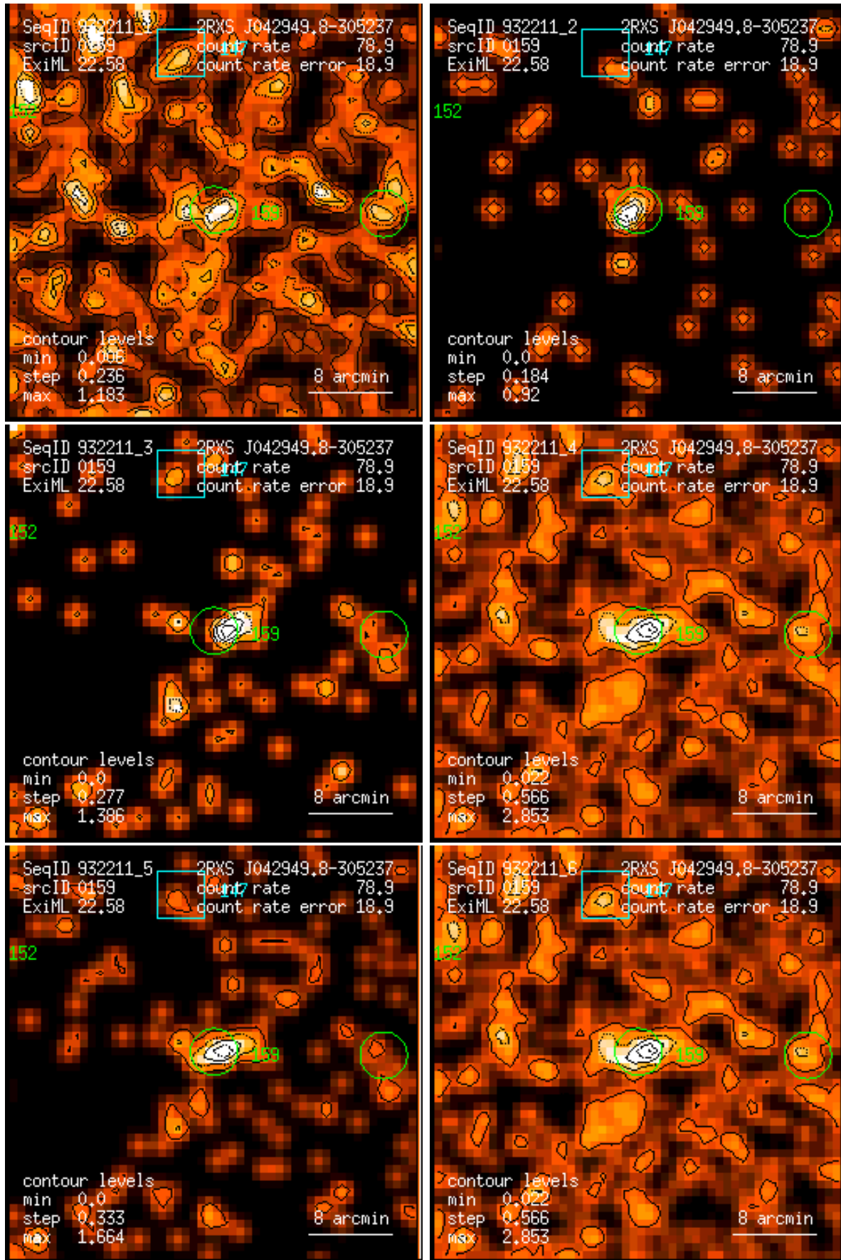
Figure 159: RASS 932211: detection 0159: band rate images, Gaussian filter: (1) PSPC channels 11 – 41, (2) 52 – 90, (3) 91 – 201, (4) 11 – 235, (5) 52 – 201, (6) 11 – 201. Broad band rates in counts/ks. Band rate contour levels in counts/ks/arcmin 2 .
