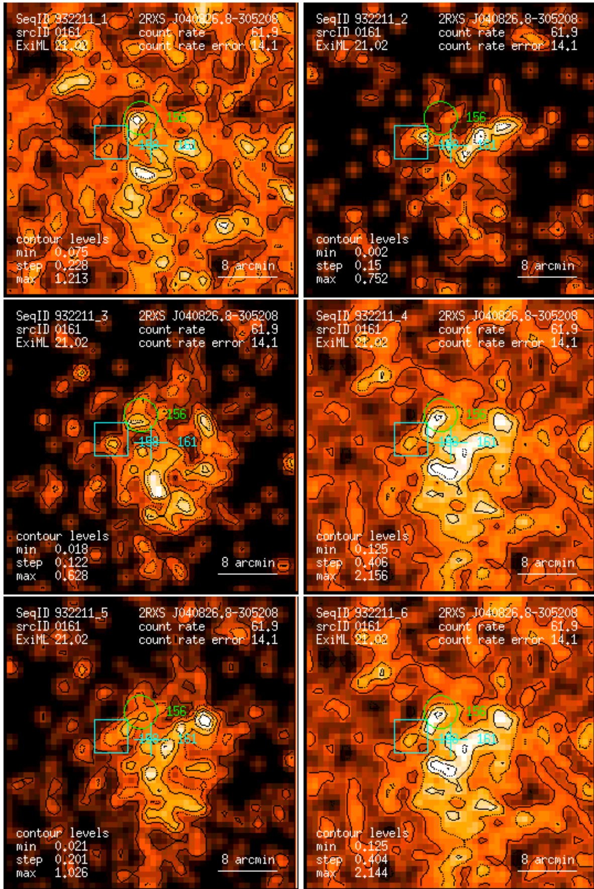
Figure 161: RASS 932211: detection 0161: band rate images, Gaussian filter: (1) PSPC channels 11 – 41, (2) 52 – 90, (3) 91 – 201, (4) 11 – 235, (5) 52 – 201, (6) 11 – 201. Broad band rates in counts/ks. Band rate contour levels in counts/ks/arcmin 2 .
