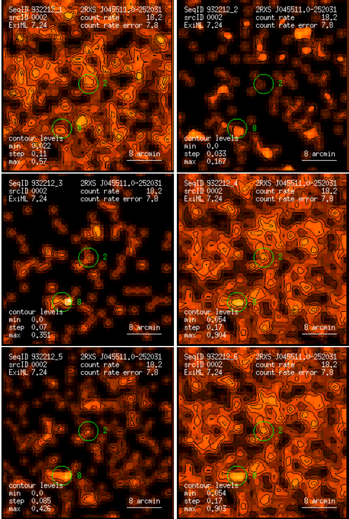
Figure 2: RASS 932212: detection 0002: band rate images, Gaussian filter: (1) PSPC channels 11 – 41, (2) 52 – 90, (3) 91 – 201, (4) 11 – 235, (5) 52 – 201, (6) 11 – 201. Broad band rates in counts/ks. Band rate contour levels in counts/ks/arcmin 2 .
