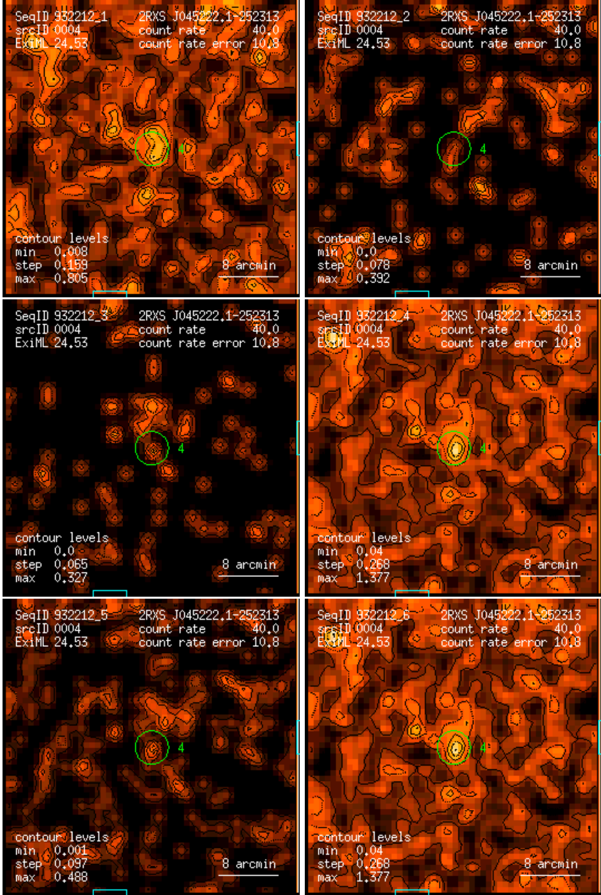
Figure 4: RASS 932212: detection 0004: band rate images, Gaussian filter: (1) PSPC channels 11 – 41, (2) 52 – 90, (3) 91 – 201, (4) 11 – 235, (5) 52 – 201, (6) 11 – 201. Broad band rates in counts/ks. Band rate contour levels in counts/ks/arcmin 2 .
