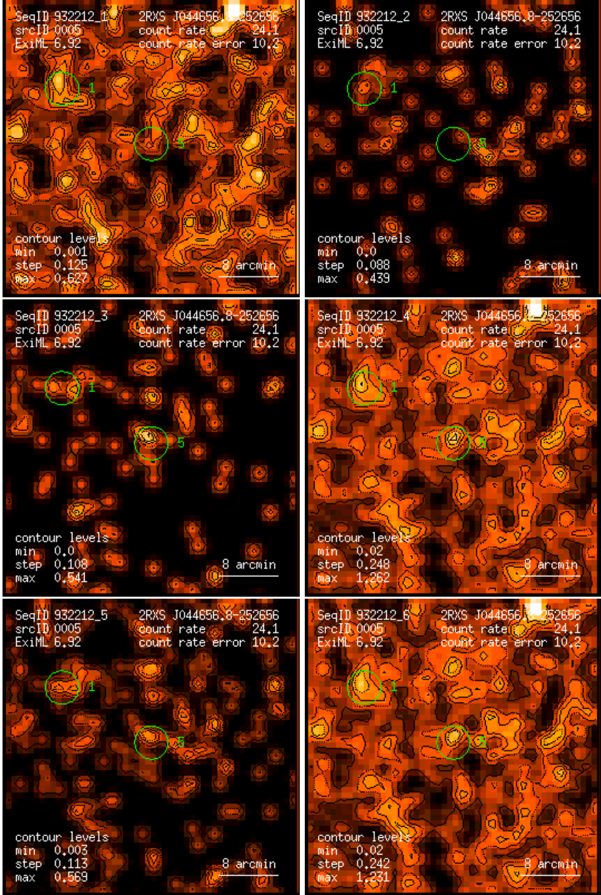
Figure 5: RASS 932212: detection 0005: band rate images, Gaussian filter: (1) PSPC channels 11 – 41, (2) 52 – 90, (3) 91 – 201, (4) 11 – 235, (5) 52 – 201, (6) 11 – 201. Broad band rates in counts/ks. Band rate contour levels in counts/ks/arcmin 2 .
