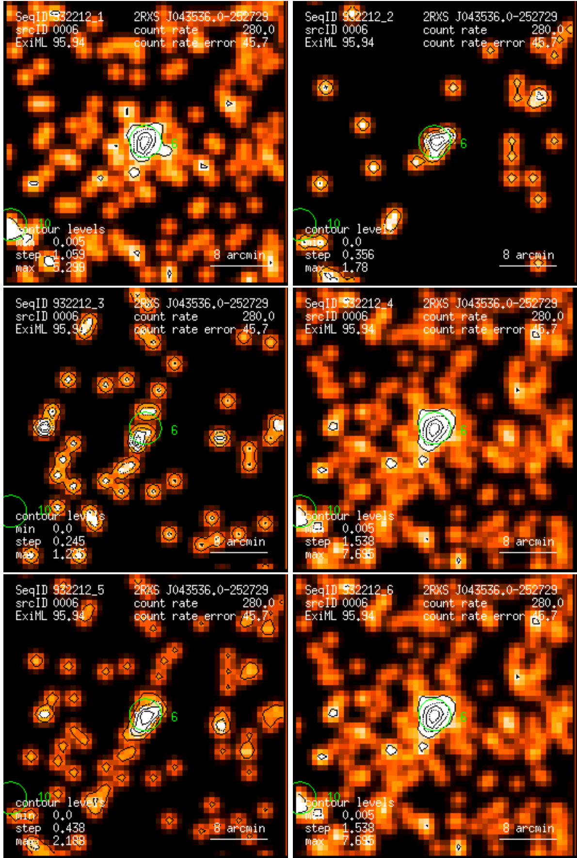
Figure 6: RASS 932212: detection 0006: band rate images, Gaussian filter: (1) PSPC channels 11 – 41, (2) 52 – 90, (3) 91 – 201, (4) 11 – 235, (5) 52 – 201, (6) 11 – 201. Broad band rates in counts/ks. Band rate contour levels in counts/ks/arcmin 2 .
