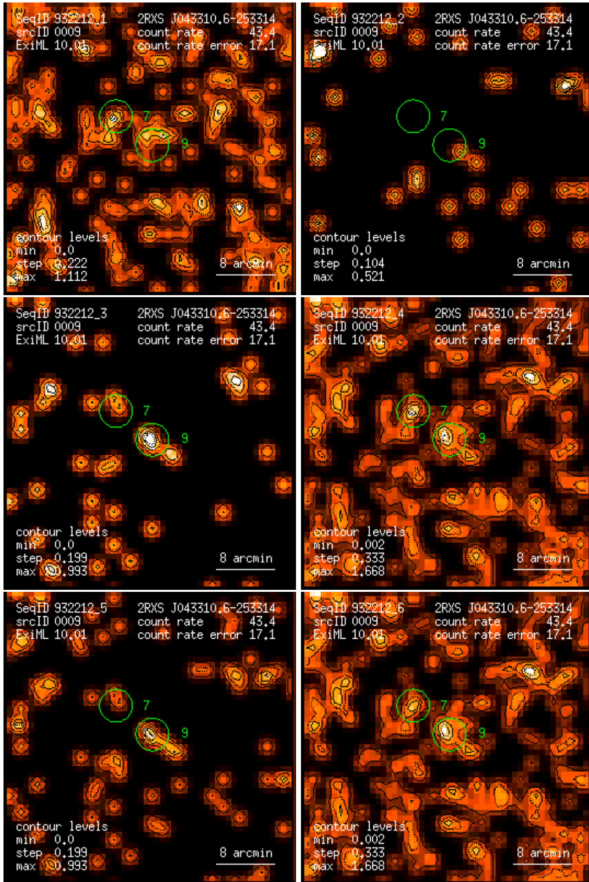
Figure 9: RASS 932212: detection 0009: band rate images, Gaussian filter: (1) PSPC channels 11 – 41, (2) 52 – 90, (3) 91 – 201, (4) 11 – 235, (5) 52 – 201, (6) 11 – 201. Broad band rates in counts/ks. Band rate contour levels in counts/ks/arcmin 2 .
