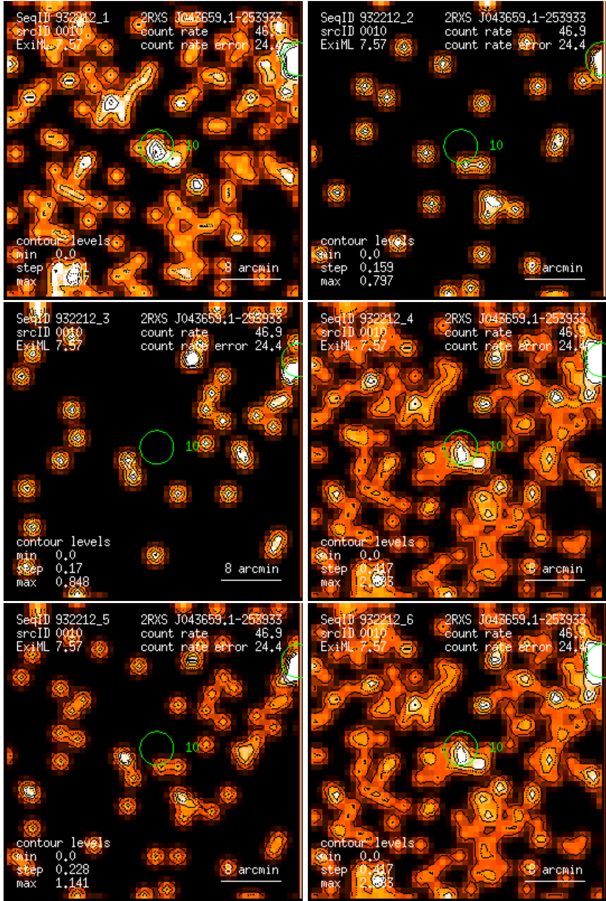
Figure 10: RASS 932212: detection 0010: band rate images, Gaussian filter: (1) PSPC channels 11 – 41, (2) 52 – 90, (3) 91 – 201, (4) 11 – 235, (5) 52 – 201, (6) 11 – 201. Broad band rates in counts/ks. Band rate contour levels in counts/ks/arcmin 2 .
