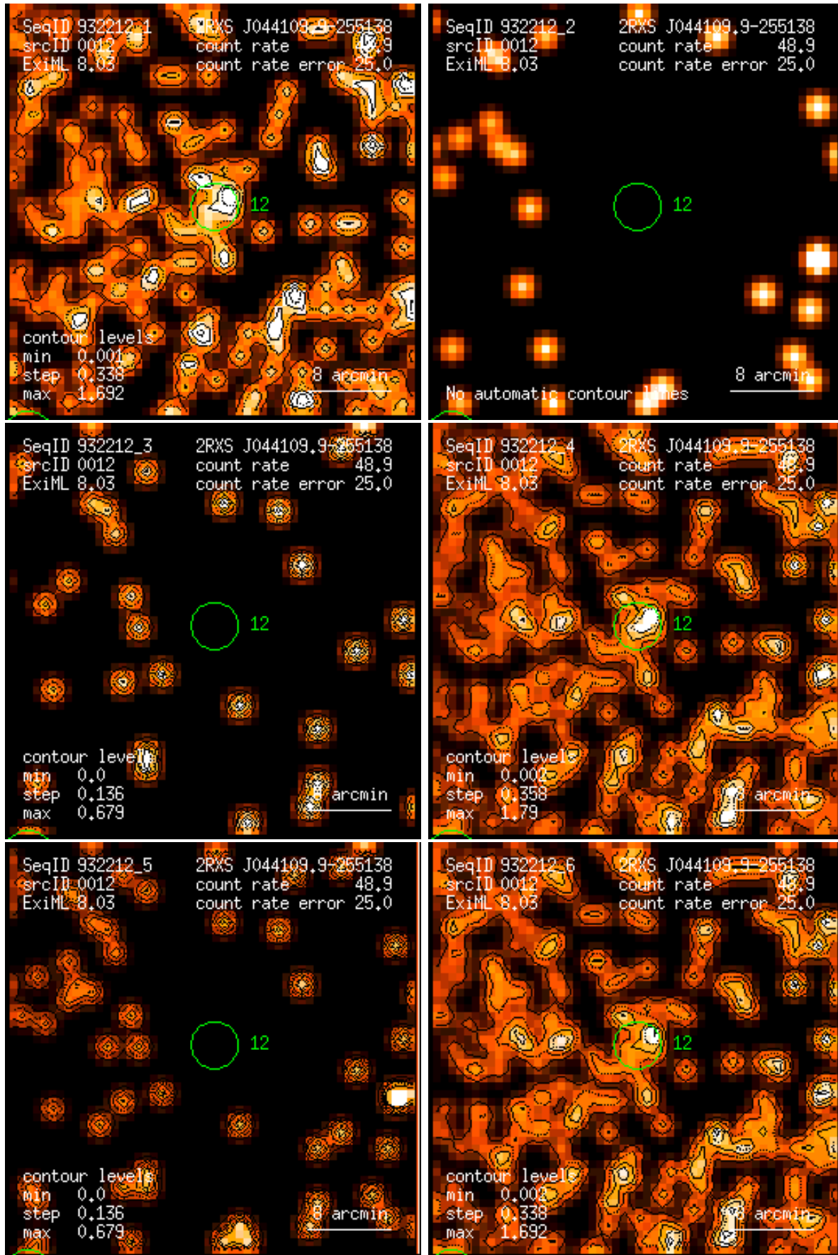
Figure 12: RASS 932212: detection 0012: band rate images, Gaussian filter: (1) PSPC channels 11 – 41, (2) 52 – 90, (3) 91 – 201, (4) 11 – 235, (5) 52 – 201, (6) 11 – 201. Broad band rates in counts/ks. Band rate contour levels in counts/ks/arcmin 2 .
