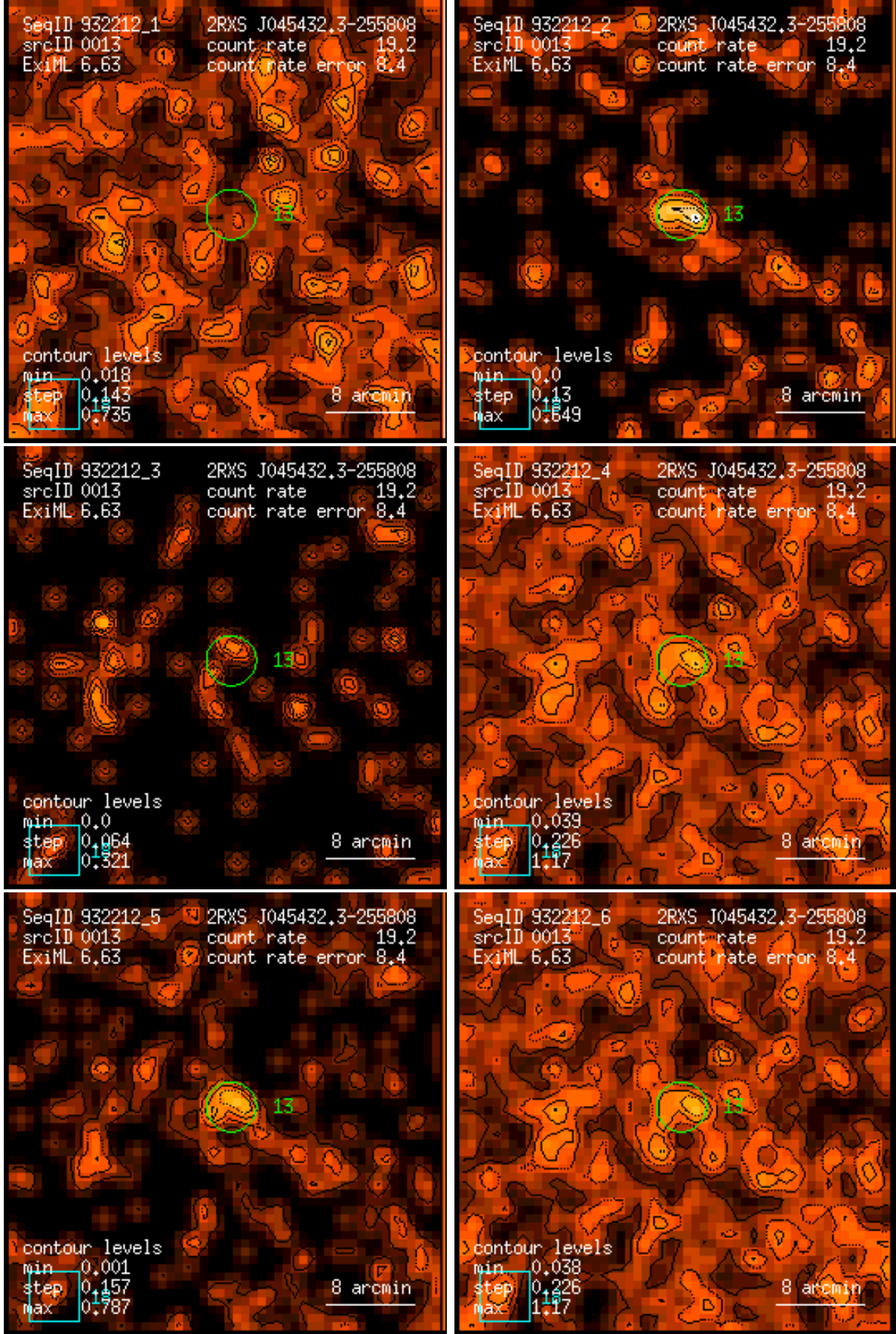
Figure 13: RASS 932212: detection 0013: band rate images, Gaussian filter: (1) PSPC channels 11 – 41, (2) 52 – 90, (3) 91 – 201, (4) 11 – 235, (5) 52 – 201, (6) 11 – 201. Broad band rates in counts/ks. Band rate contour levels in counts/ks/arcmin 2 .
