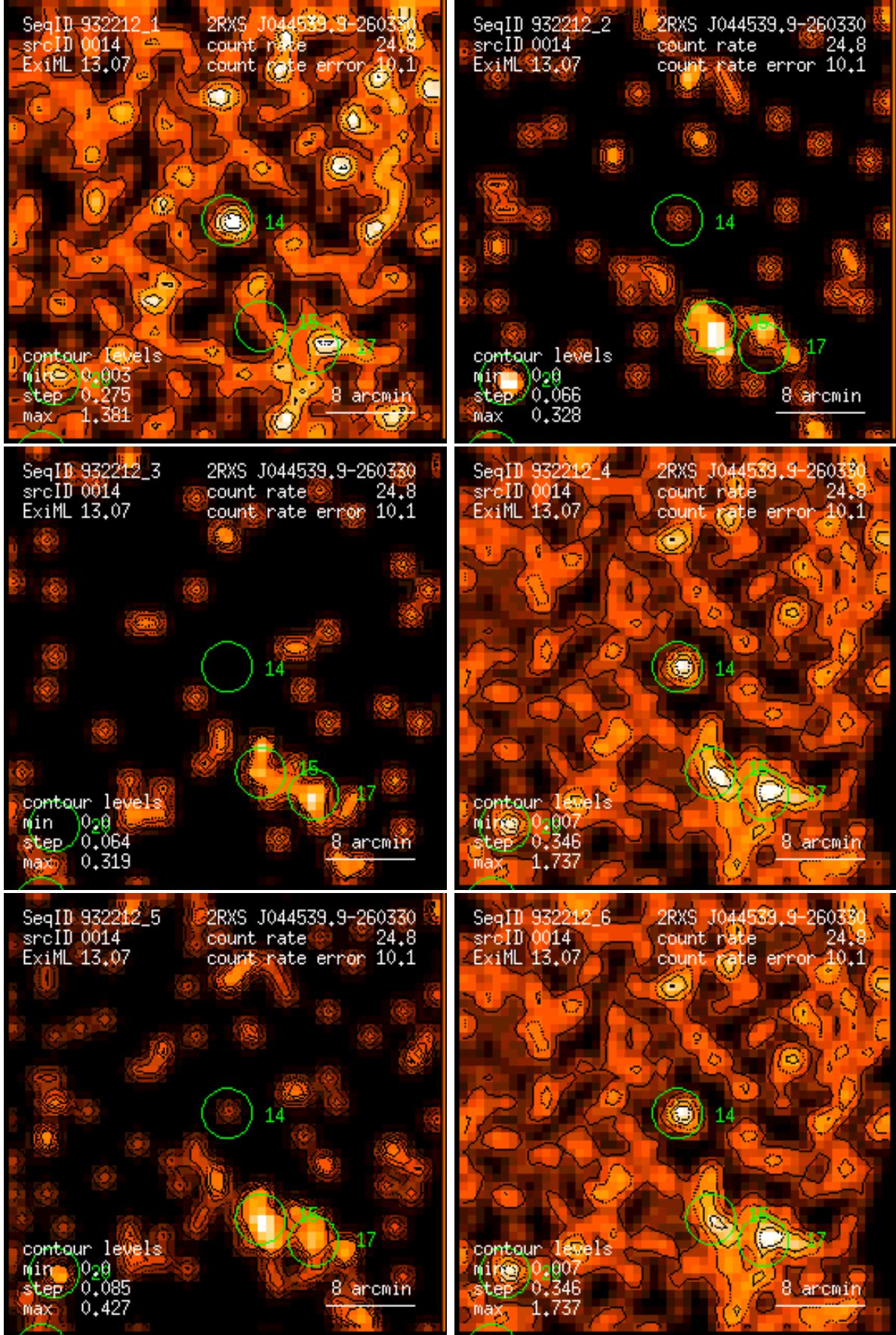
Figure 14: RASS 932212: detection 0014: band rate images, Gaussian filter: (1) PSPC channels 11 – 41, (2) 52 – 90, (3) 91 – 201, (4) 11 – 235, (5) 52 – 201, (6) 11 – 201. Broad band rates in counts/ks. Band rate contour levels in counts/ks/arcmin 2 .
