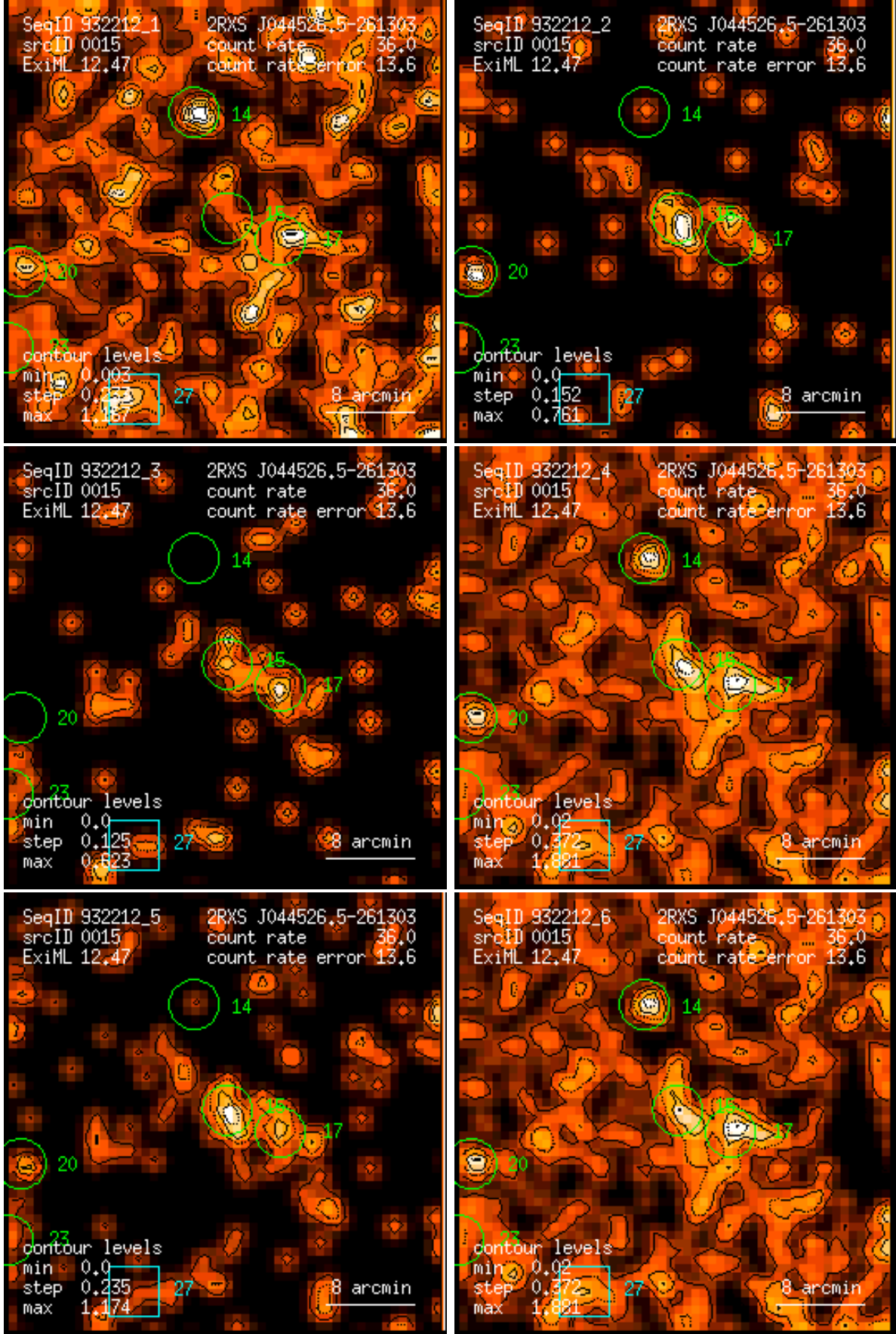
Figure 15: RASS 932212: detection 0015: band rate images, Gaussian filter: (1) PSPC channels 11 – 41, (2) 52 – 90, (3) 91 – 201, (4) 11 – 235, (5) 52 – 201, (6) 11 – 201. Broad band rates in counts/ks. Band rate contour levels in counts/ks/arcmin 2 .
