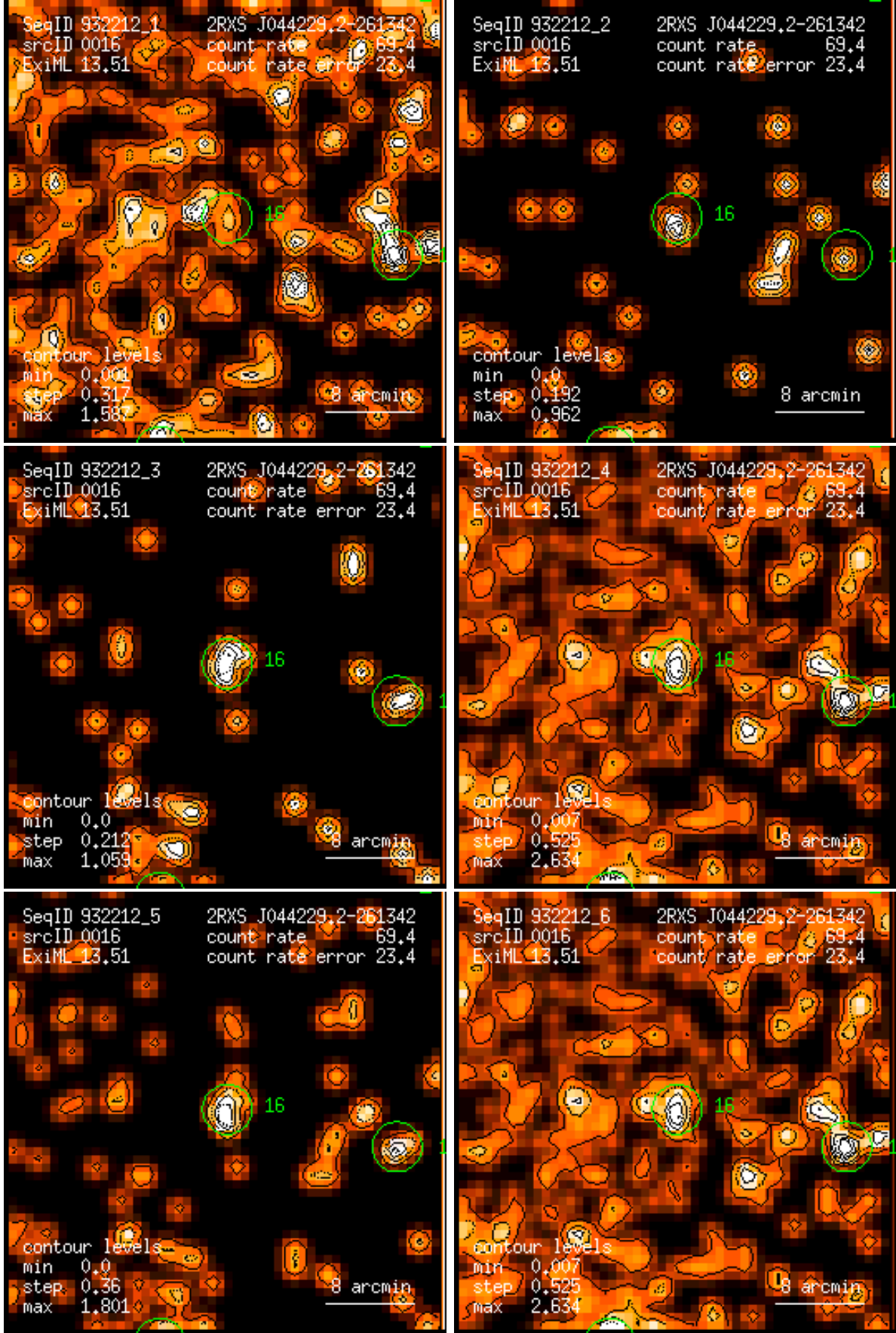
Figure 16: RASS 932212: detection 0016: band rate images, Gaussian filter: (1) PSPC channels 11 – 41, (2) 52 – 90, (3) 91 – 201, (4) 11 – 235, (5) 52 – 201, (6) 11 – 201. Broad band rates in counts/ks. Band rate contour levels in counts/ks/arcmin 2 .
