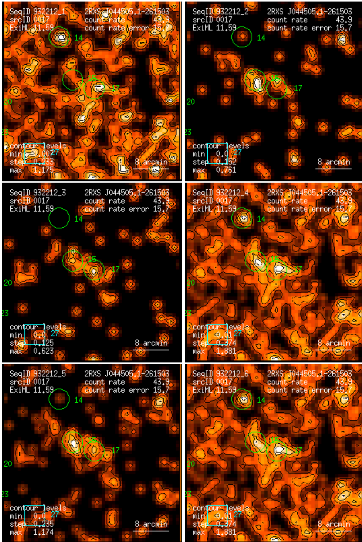
Figure 17: RASS 932212: detection 0017: band rate images, Gaussian filter: (1) PSPC channels 11 – 41, (2) 52 – 90, (3) 91 – 201, (4) 11 – 235, (5) 52 – 201, (6) 11 – 201. Broad band rates in counts/ks. Band rate contour levels in counts/ks/arcmin 2 .
