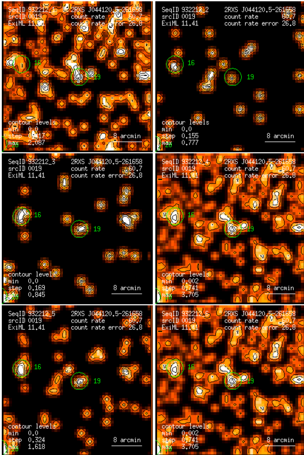
Figure 19: RASS 932212: detection 0019: band rate images, Gaussian filter: (1) PSPC channels 11 – 41, (2) 52 – 90, (3) 91 – 201, (4) 11 – 235, (5) 52 – 201, (6) 11 – 201. Broad band rates in counts/ks. Band rate contour levels in counts/ks/arcmin 2 .
