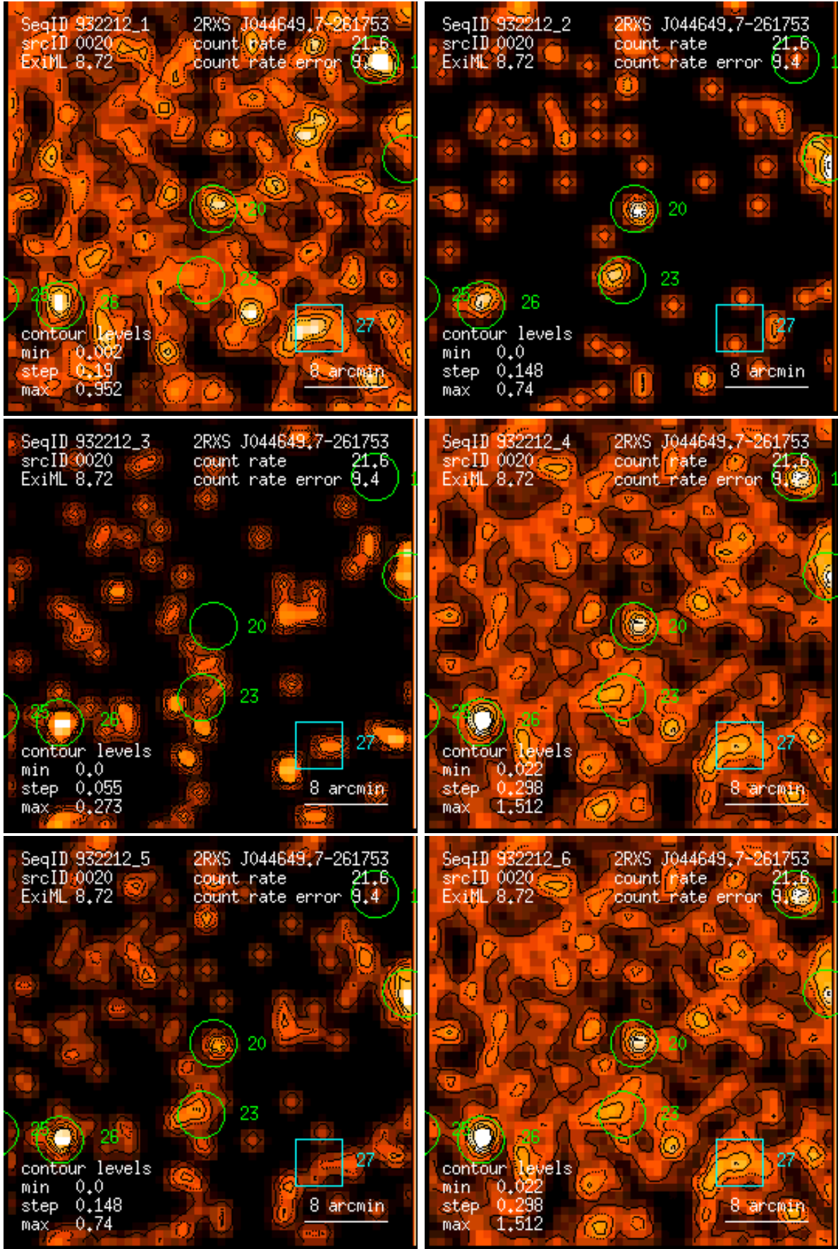
Figure 20: RASS 932212: detection 0020: band rate images, Gaussian filter: (1) PSPC channels 11 – 41, (2) 52 – 90, (3) 91 – 201, (4) 11 – 235, (5) 52 – 201, (6) 11 – 201. Broad band rates in counts/ks. Band rate contour levels in counts/ks/arcmin 2 .
