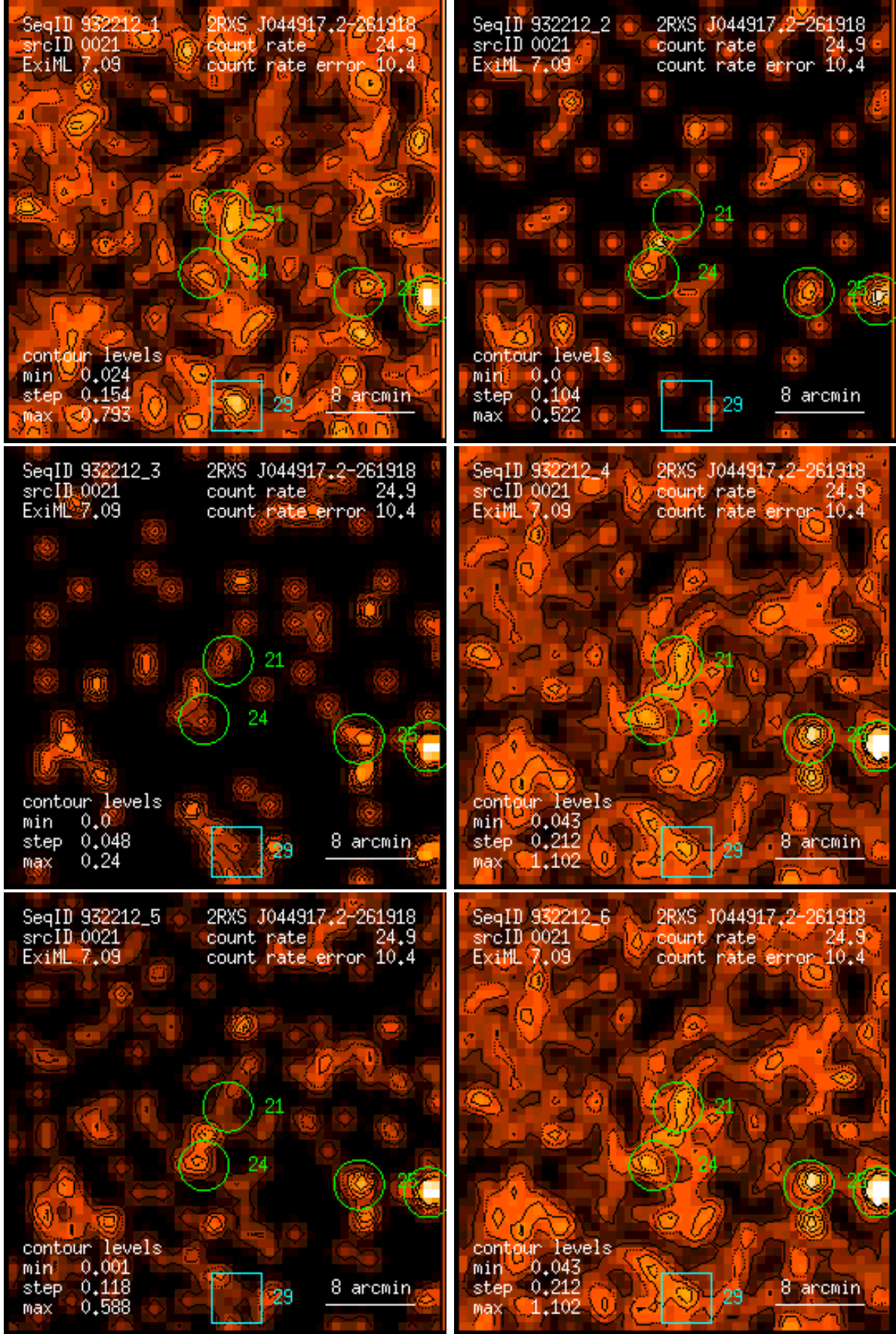
Figure 21: RASS 932212: detection 0021: band rate images, Gaussian filter: (1) PSPC channels 11 – 41, (2) 52 – 90, (3) 91 – 201, (4) 11 – 235, (5) 52 – 201, (6) 11 – 201. Broad band rates in counts/ks. Band rate contour levels in counts/ks/arcmin 2 .
