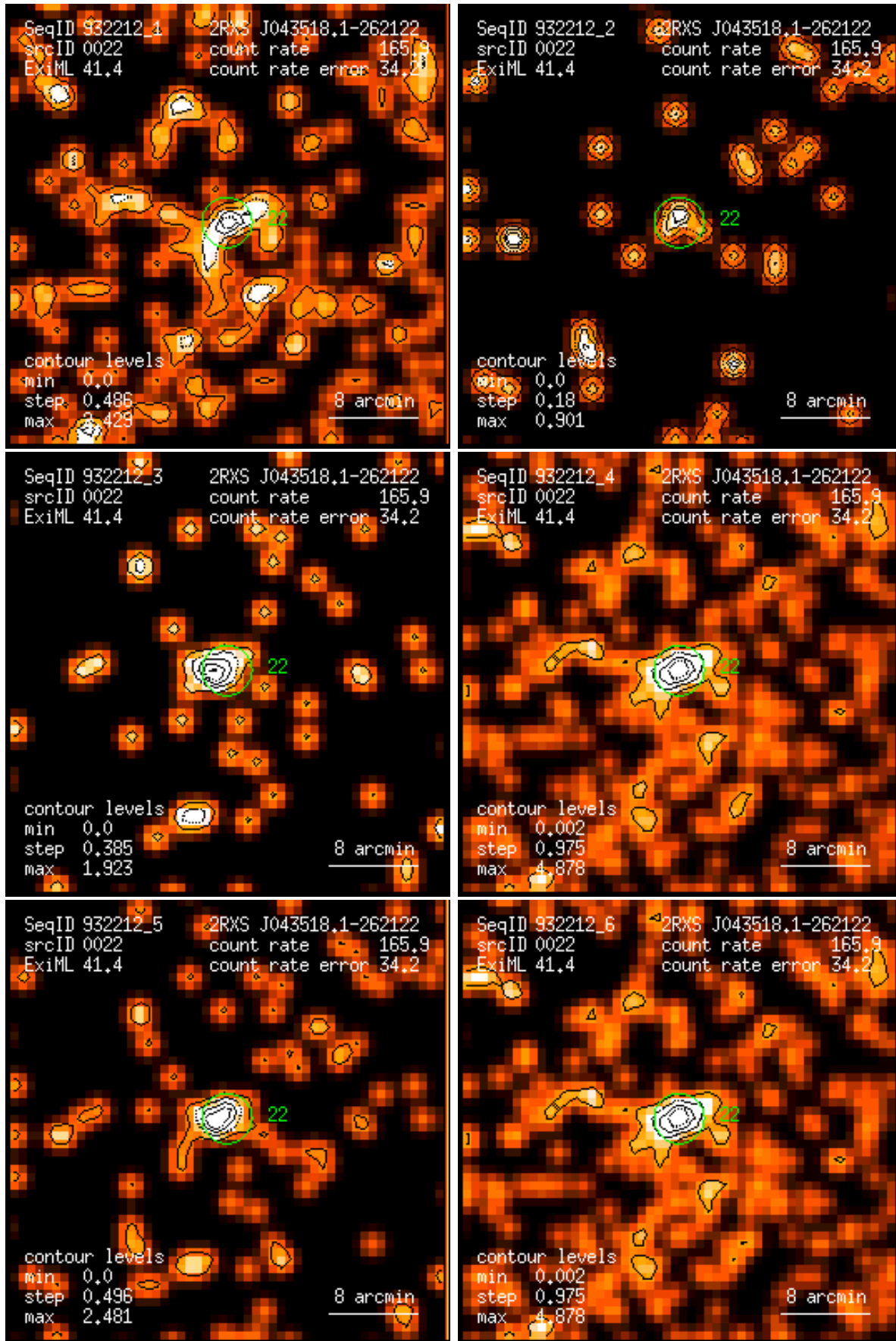
Figure 22: RASS 932212: detection 0022: band rate images, Gaussian filter: (1) PSPC channels 11 – 41, (2) 52 – 90, (3) 91 – 201, (4) 11 – 235, (5) 52 – 201, (6) 11 – 201. Broad band rates in counts/ks. Band rate contour levels in counts/ks/arcmin 2 .
