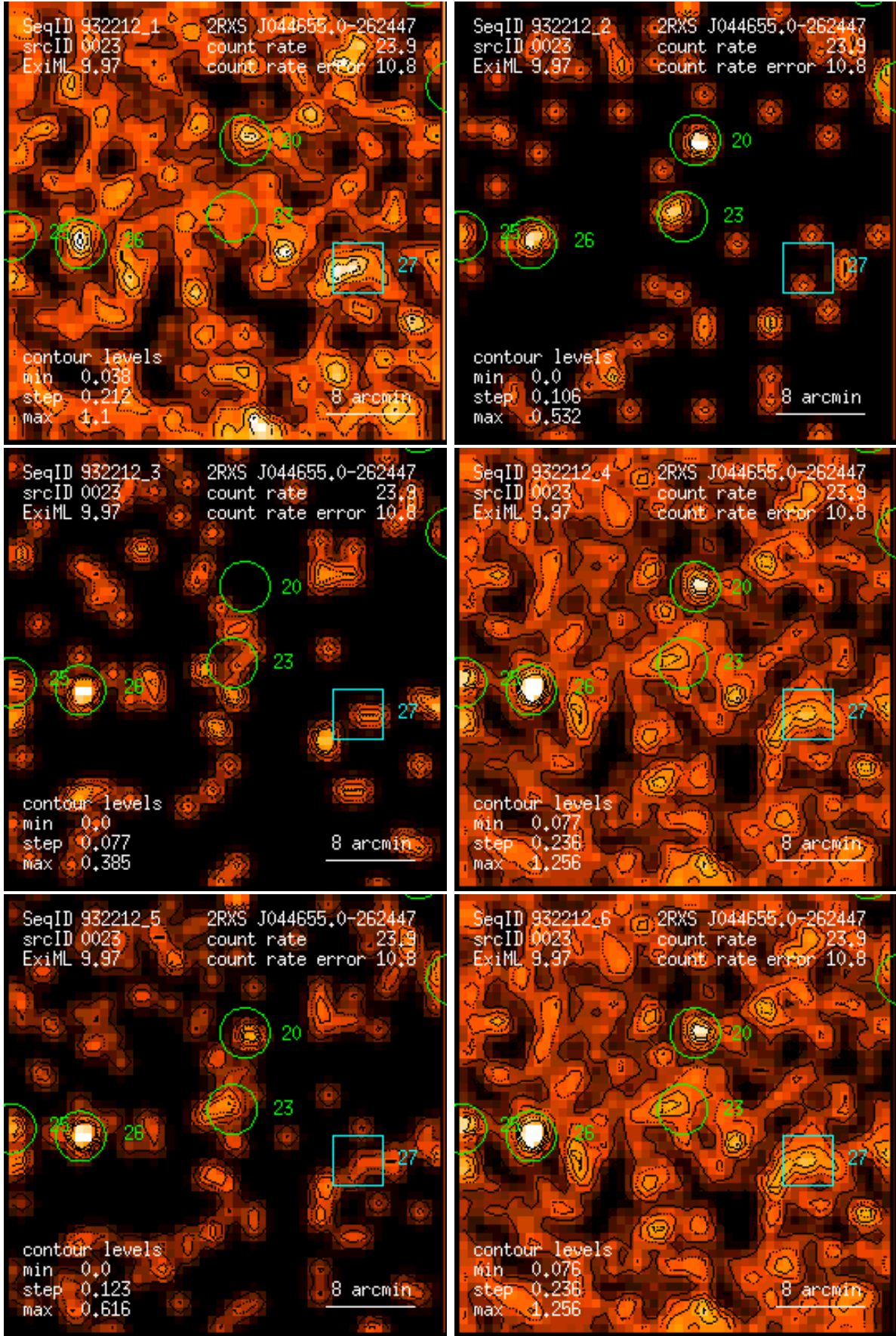
Figure 23: RASS 932212: detection 0023: band rate images, Gaussian filter: (1) PSPC channels 11 – 41, (2) 52 – 90, (3) 91 – 201, (4) 11 – 235, (5) 52 – 201, (6) 11 – 201. Broad band rates in counts/ks. Band rate contour levels in counts/ks/arcmin 2 .
