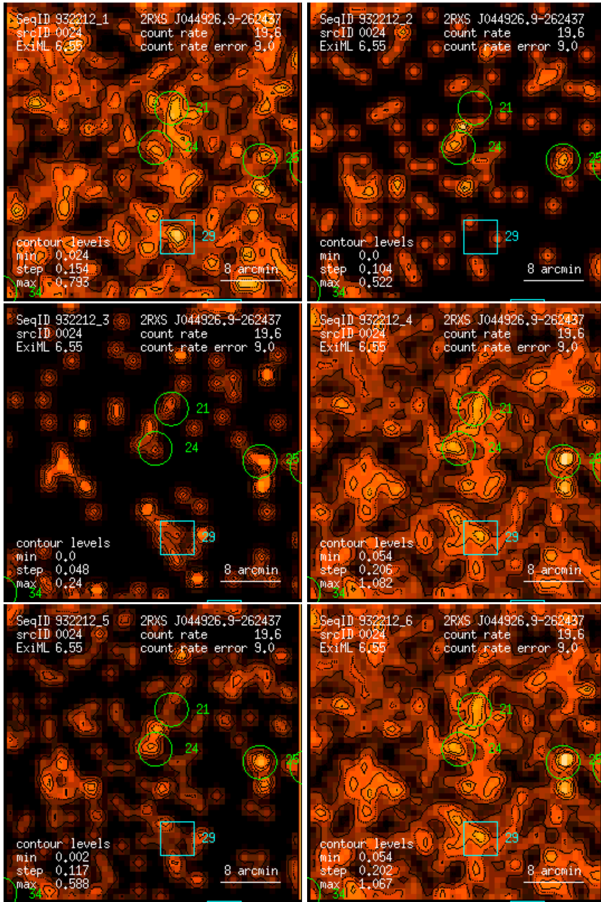
Figure 24: RASS 932212: detection 0024: band rate images, Gaussian filter: (1) PSPC channels 11 – 41, (2) 52 – 90, (3) 91 – 201, (4) 11 – 235, (5) 52 – 201, (6) 11 – 201. Broad band rates in counts/ks. Band rate contour levels in counts/ks/arcmin 2 .
