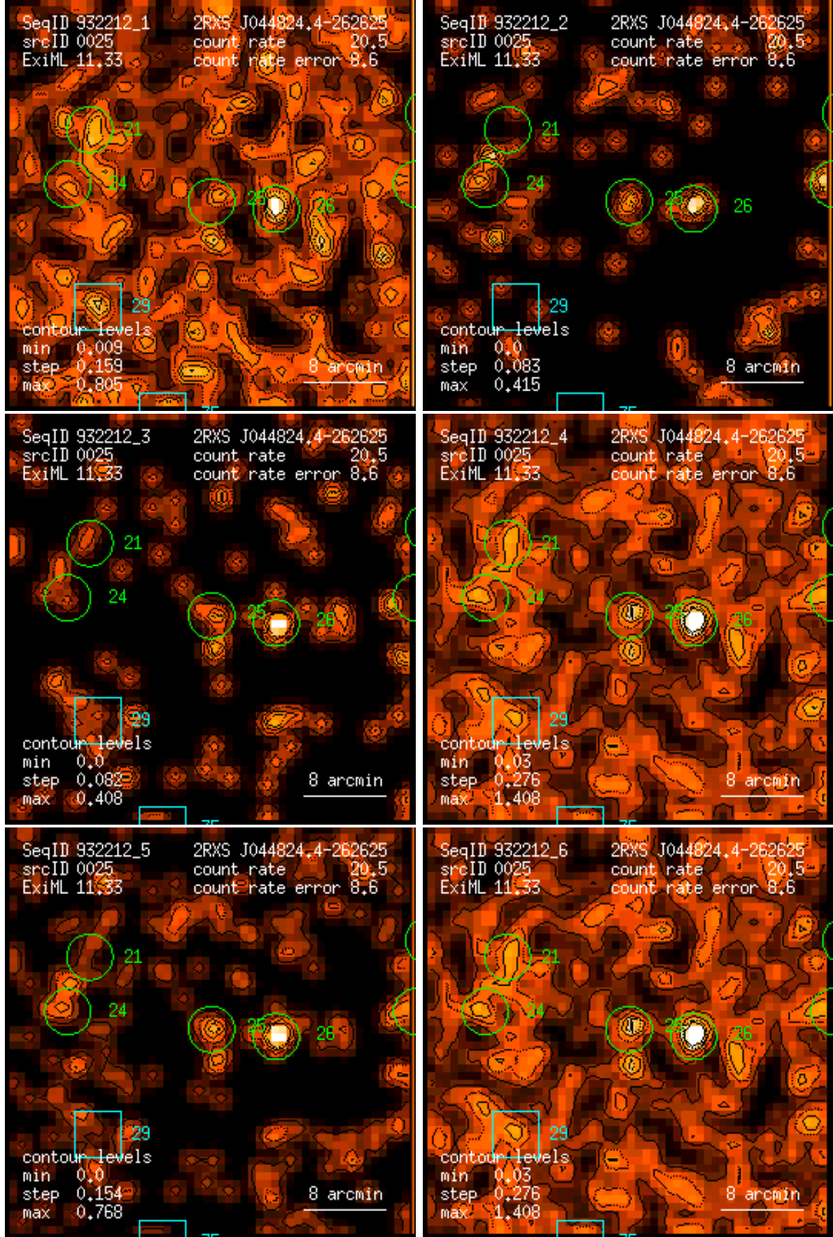
Figure 25: RASS 932212: detection 0025: band rate images, Gaussian filter: (1) PSPC channels 11 – 41, (2) 52 – 90, (3) 91 – 201, (4) 11 – 235, (5) 52 – 201, (6) 11 – 201. Broad band rates in counts/ks. Band rate contour levels in counts/ks/arcmin 2 .
