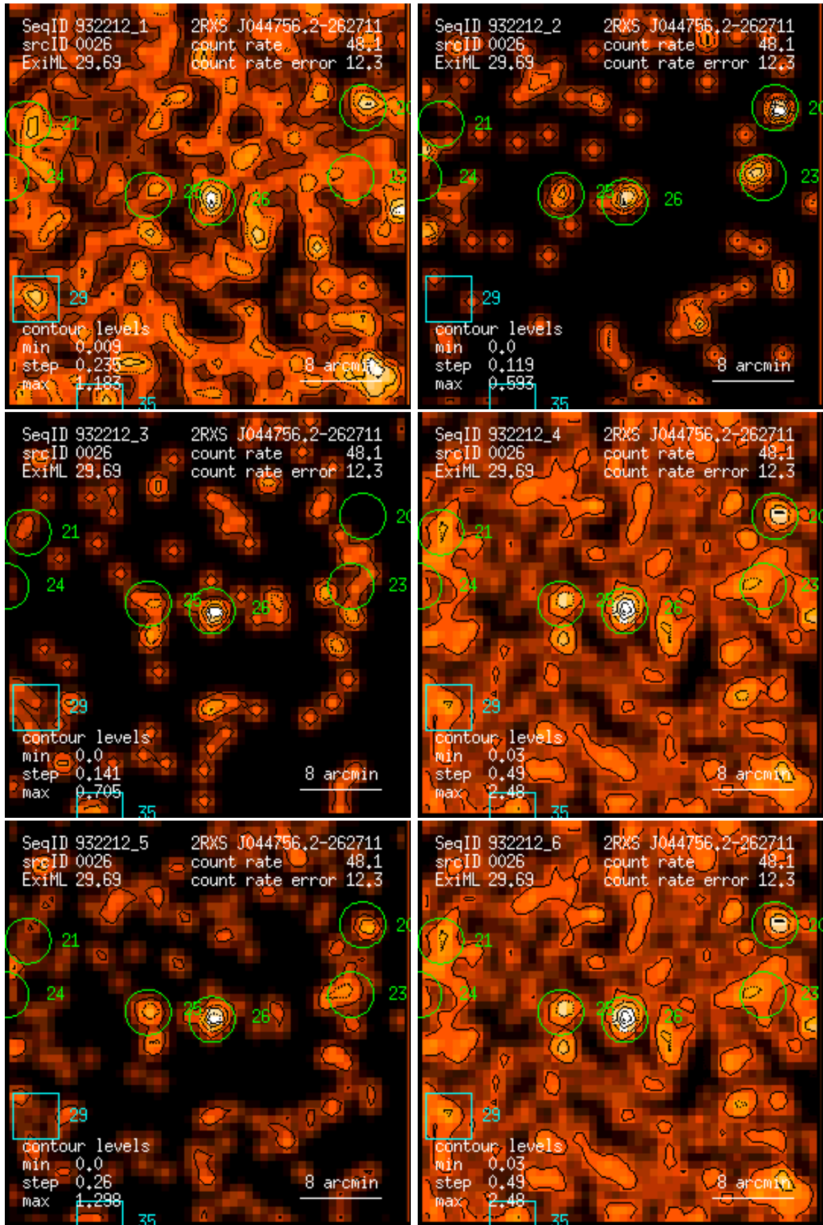
Figure 26: RASS 932212: detection 0026: band rate images, Gaussian filter: (1) PSPC channels 11 – 41, (2) 52 – 90, (3) 91 – 201, (4) 11 – 235, (5) 52 – 201, (6) 11 – 201. Broad band rates in counts/ks. Band rate contour levels in counts/ks/arcmin 2 .
