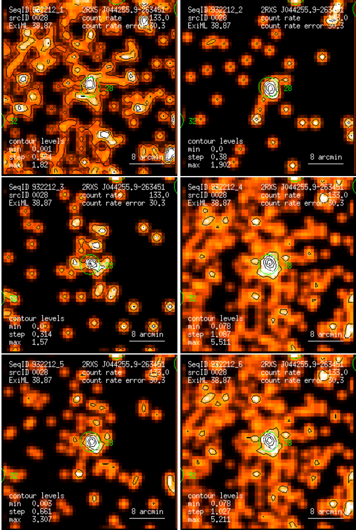
Figure 28: RASS 932212: detection 0028: band rate images, Gaussian filter: (1) PSPC channels 11 – 41, (2) 52 – 90, (3) 91 – 201, (4) 11 – 235, (5) 52 – 201, (6) 11 – 201. Broad band rates in counts/ks. Band rate contour levels in counts/ks/arcmin 2 .
