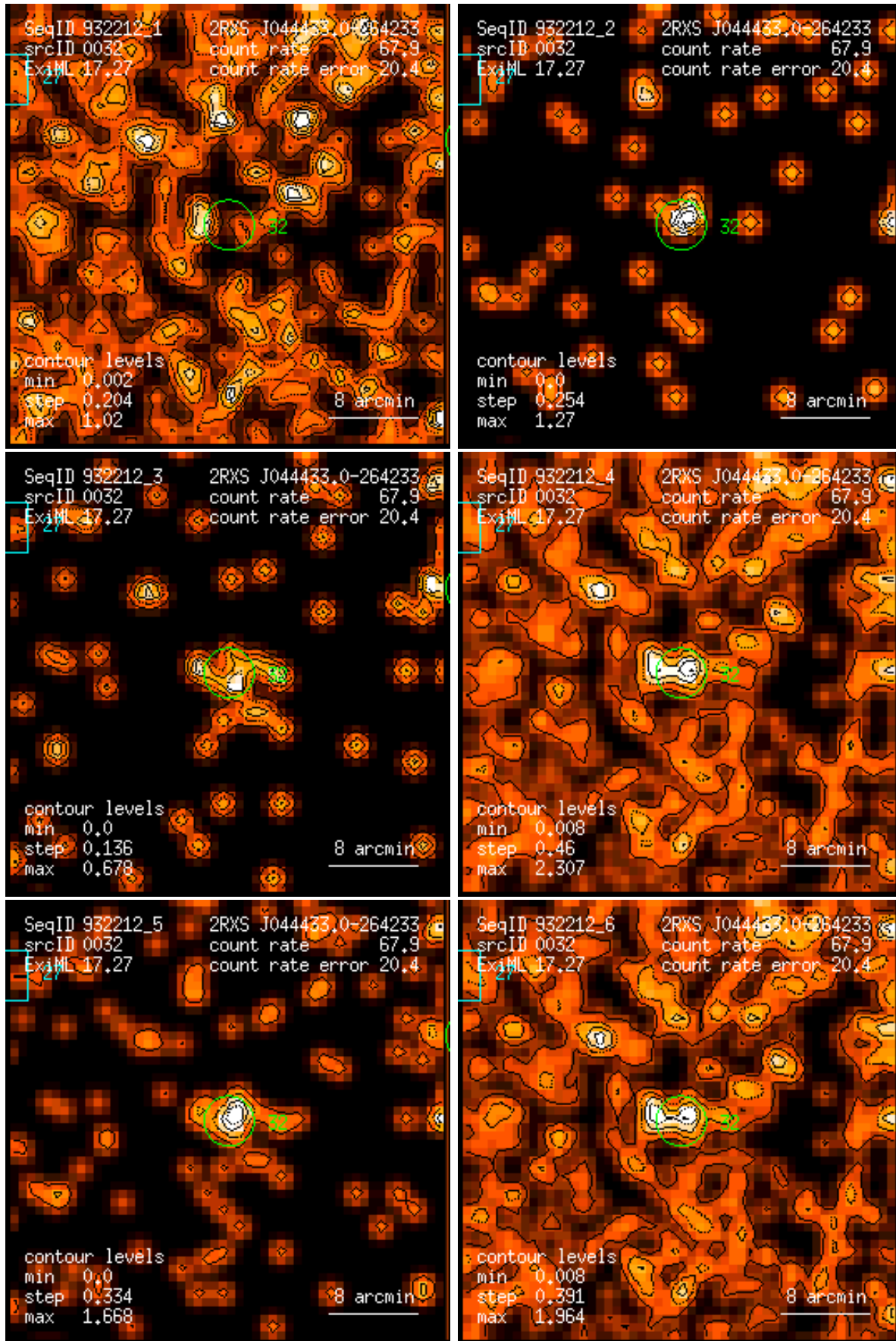
Figure 32: RASS 932212: detection 0032: band rate images, Gaussian filter: (1) PSPC channels 11 – 41, (2) 52 – 90, (3) 91 – 201, (4) 11 – 235, (5) 52 – 201, (6) 11 – 201. Broad band rates in counts/ks. Band rate contour levels in counts/ks/arcmin 2 .
