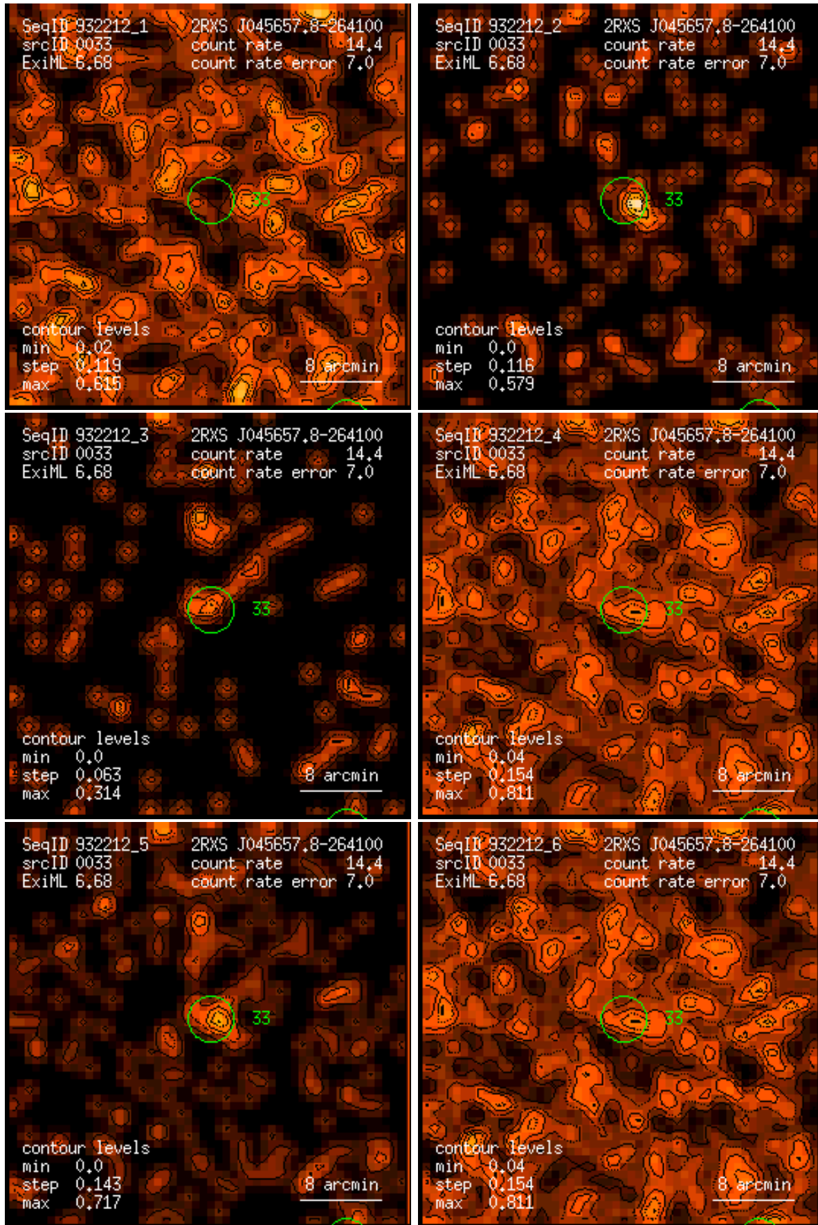
Figure 33: RASS 932212: detection 0033: band rate images, Gaussian filter: (1) PSPC channels 11 – 41, (2) 52 – 90, (3) 91 – 201, (4) 11 – 235, (5) 52 – 201, (6) 11 – 201. Broad band rates in counts/ks. Band rate contour levels in counts/ks/arcmin 2 .
