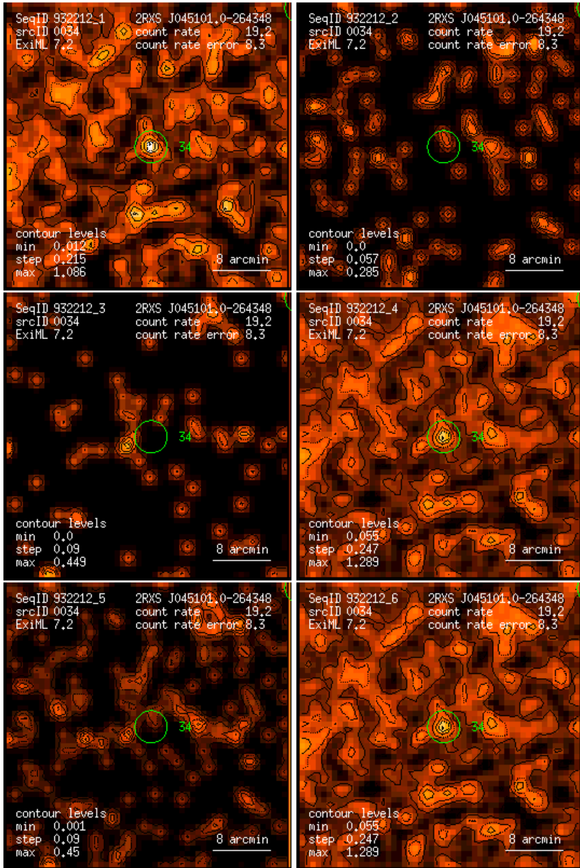
Figure 34: RASS 932212: detection 0034: band rate images, Gaussian filter: (1) PSPC channels 11 – 41, (2) 52 – 90, (3) 91 – 201, (4) 11 – 235, (5) 52 – 201, (6) 11 – 201. Broad band rates in counts/ks. Band rate contour levels in counts/ks/arcmin 2 .
