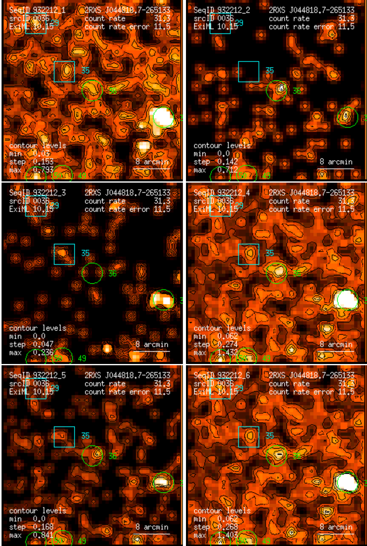
Figure 36: RASS 932212: detection 0036: band rate images, Gaussian filter: (1) PSPC channels 11 – 41, (2) 52 – 90, (3) 91 – 201, (4) 11 – 235, (5) 52 – 201, (6) 11 – 201. Broad band rates in counts/ks. Band rate contour levels in counts/ks/arcmin 2 .
