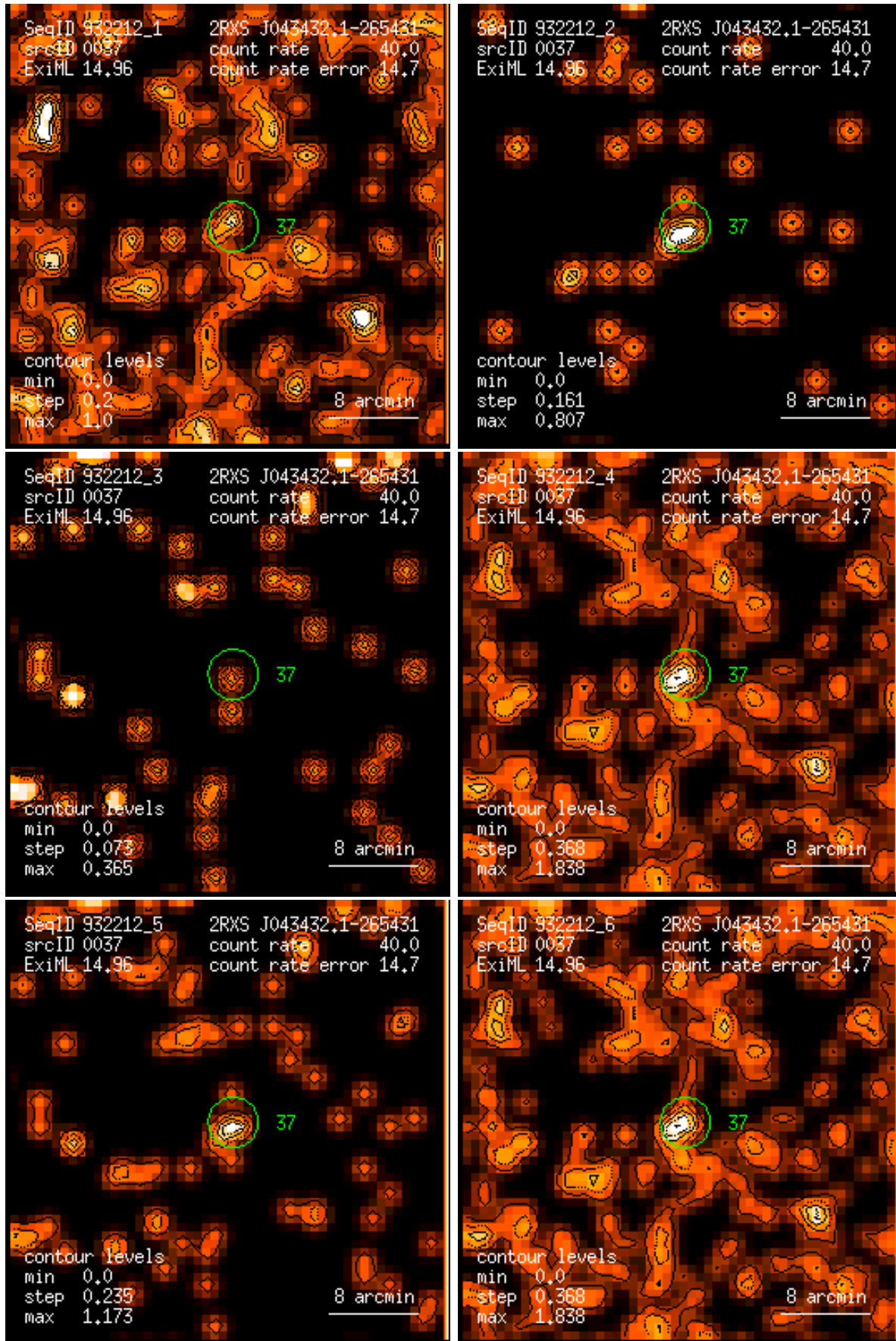
Figure 37: RASS 932212: detection 0037: band rate images, Gaussian filter: (1) PSPC channels 11 – 41, (2) 52 – 90, (3) 91 – 201, (4) 11 – 235, (5) 52 – 201, (6) 11 – 201. Broad band rates in counts/ks. Band rate contour levels in counts/ks/arcmin 2 .
