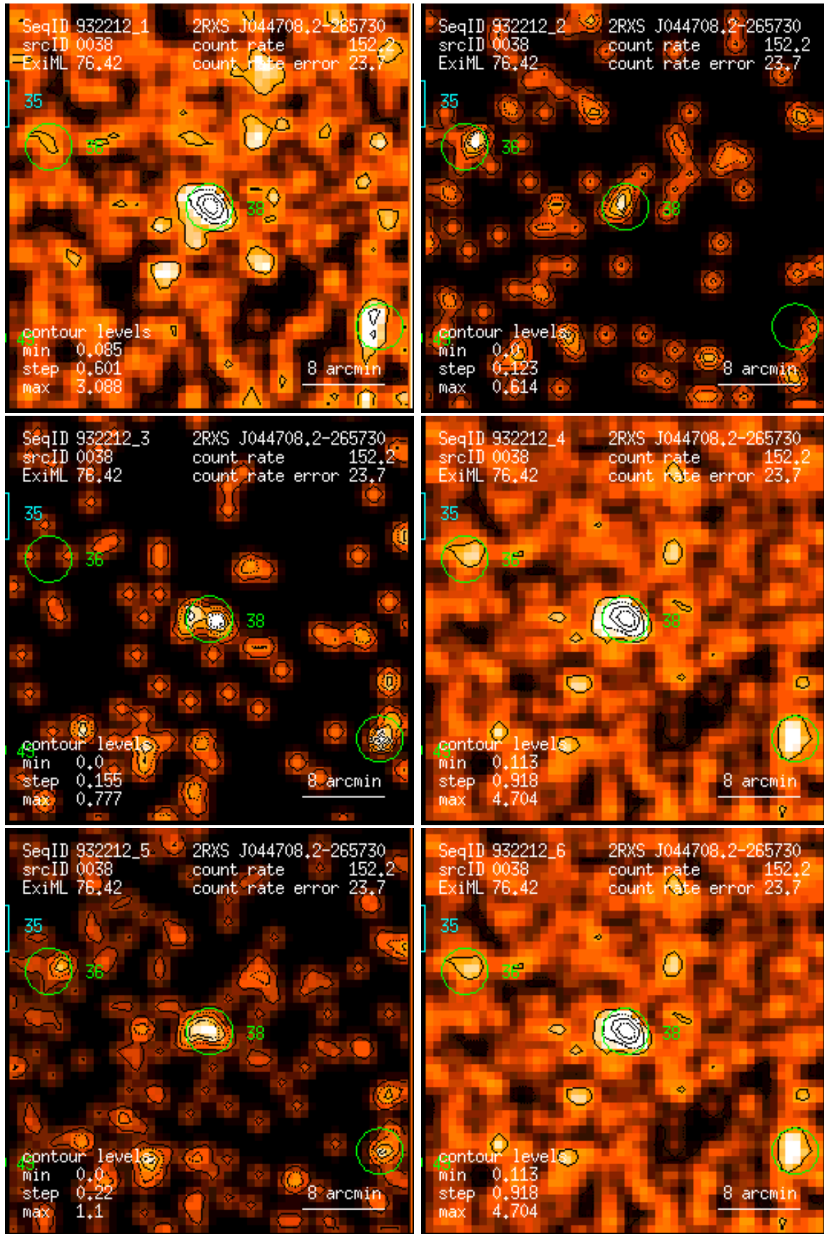
Figure 38: RASS 932212: detection 0038: band rate images, Gaussian filter: (1) PSPC channels 11 – 41, (2) 52 – 90, (3) 91 – 201, (4) 11 – 235, (5) 52 – 201, (6) 11 – 201. Broad band rates in counts/ks. Band rate contour levels in counts/ks/arcmin 2 .
