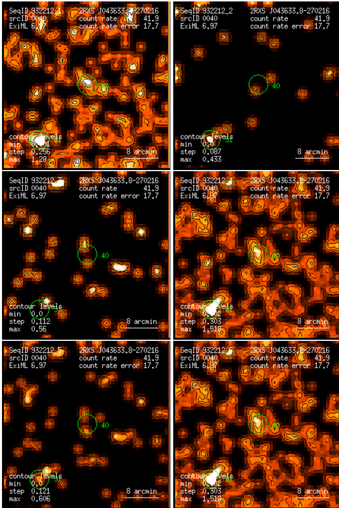
Figure 40: RASS 932212: detection 0040: band rate images, Gaussian filter: (1) PSPC channels 11 – 41, (2) 52 – 90, (3) 91 – 201, (4) 11 – 235, (5) 52 – 201, (6) 11 – 201. Broad band rates in counts/ks. Band rate contour levels in counts/ks/arcmin 2 .
