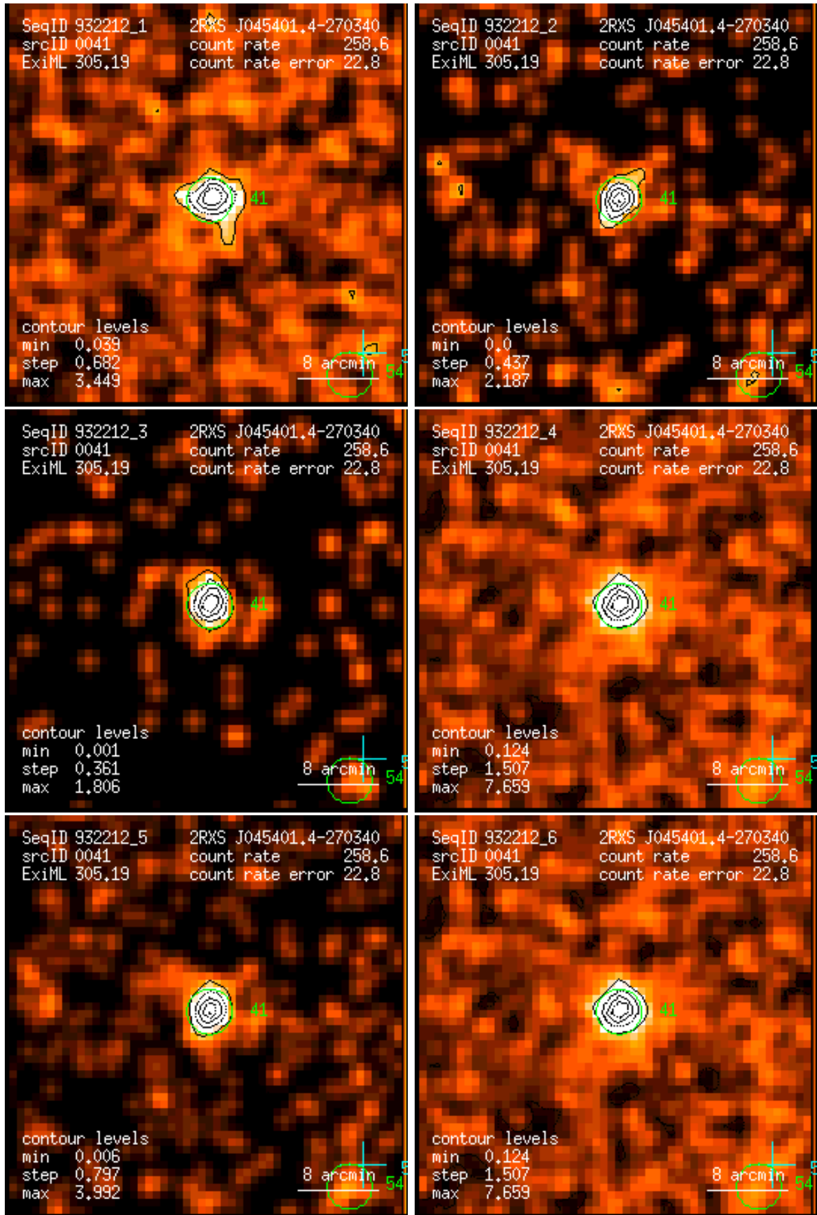
Figure 41: RASS 932212: detection 0041: band rate images, Gaussian filter: (1) PSPC channels 11 – 41, (2) 52 – 90, (3) 91 – 201, (4) 11 – 235, (5) 52 – 201, (6) 11 – 201. Broad band rates in counts/ks. Band rate contour levels in counts/ks/arcmin 2 .
