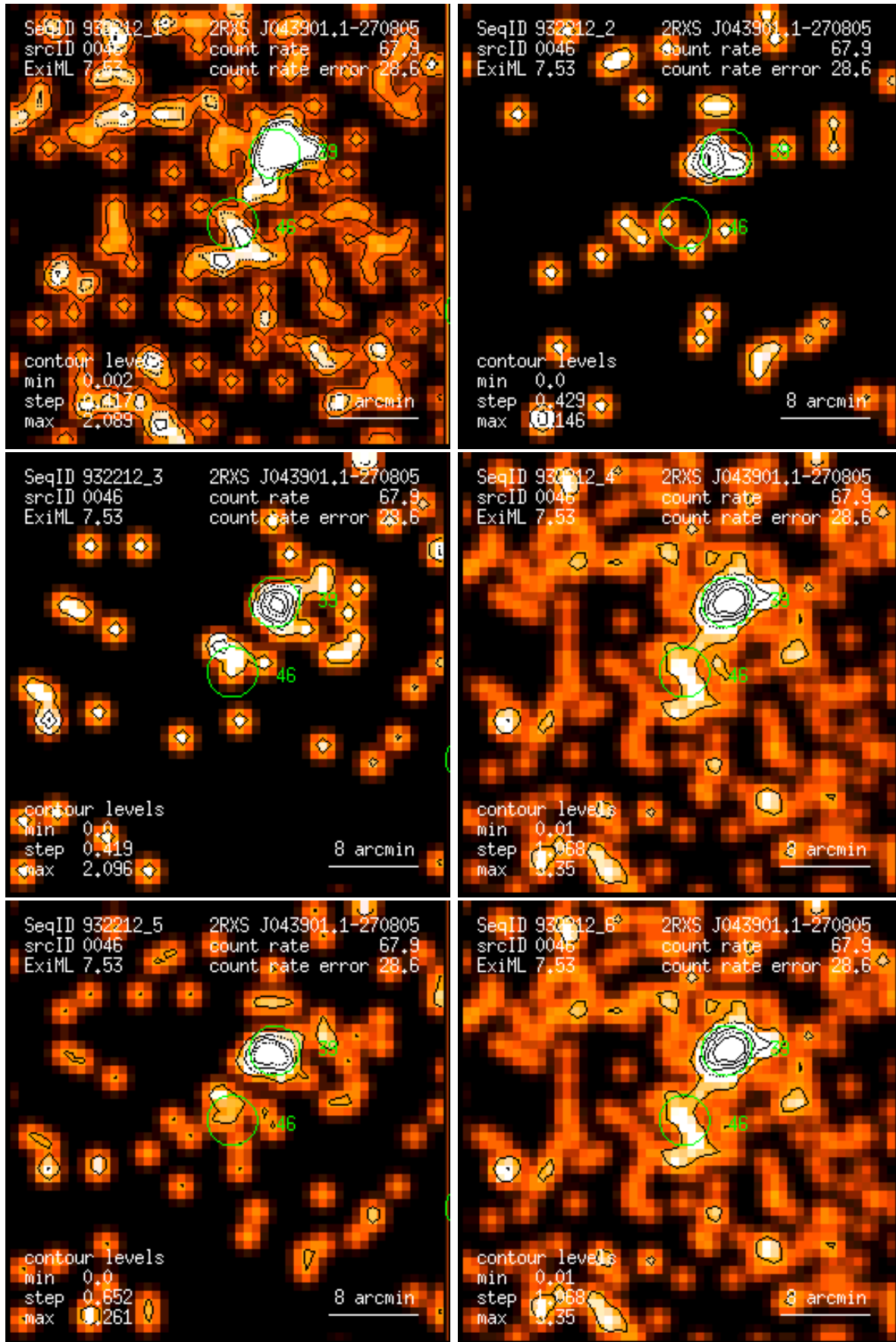
Figure 46: RASS 932212: detection 0046: band rate images, Gaussian filter: (1) PSPC channels 11 – 41, (2) 52 – 90, (3) 91 – 201, (4) 11 – 235, (5) 52 – 201, (6) 11 – 201. Broad band rates in counts/ks. Band rate contour levels in counts/ks/arcmin 2 .
