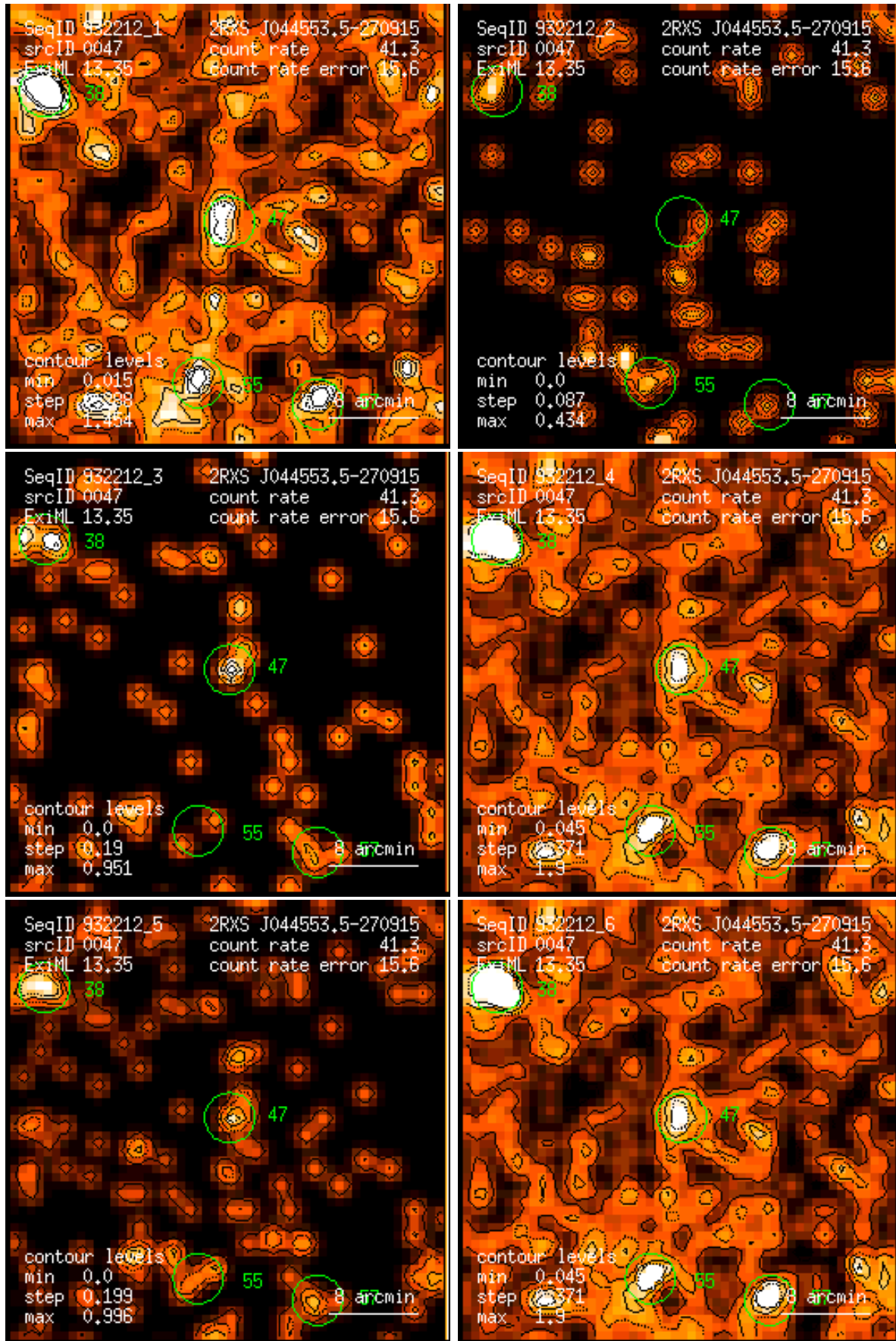
Figure 47: RASS 932212: detection 0047: band rate images, Gaussian filter: (1) PSPC channels 11 – 41, (2) 52 – 90, (3) 91 – 201, (4) 11 – 235, (5) 52 – 201, (6) 11 – 201. Broad band rates in counts/ks. Band rate contour levels in counts/ks/arcmin 2 .
