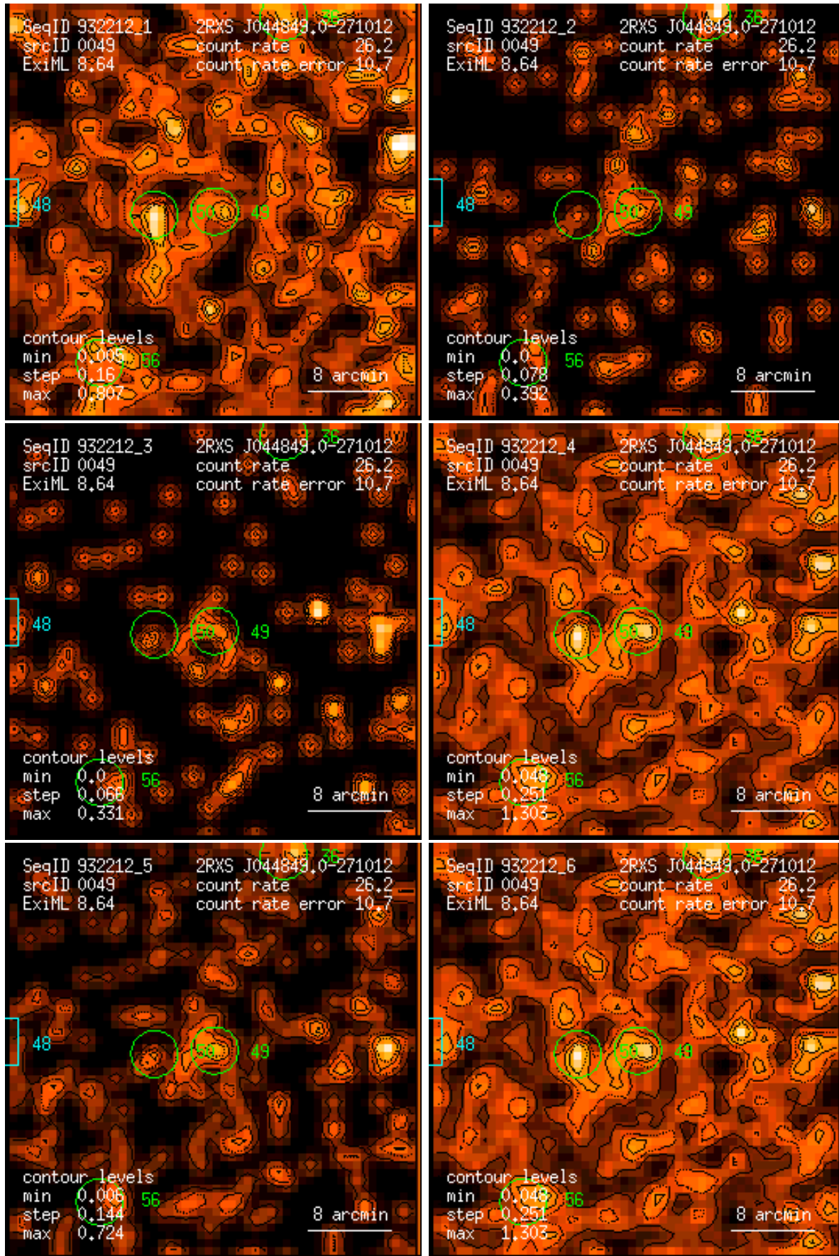
Figure 49: RASS 932212: detection 0049: band rate images, Gaussian filter: (1) PSPC channels 11 – 41, (2) 52 – 90, (3) 91 – 201, (4) 11 – 235, (5) 52 – 201, (6) 11 – 201. Broad band rates in counts/ks. Band rate contour levels in counts/ks/arcmin 2 .
