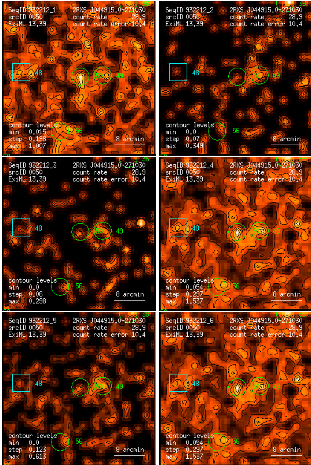
Figure 50: RASS 932212: detection 0050: band rate images, Gaussian filter: (1) PSPC channels 11 – 41, (2) 52 – 90, (3) 91 – 201, (4) 11 – 235, (5) 52 – 201, (6) 11 – 201. Broad band rates in counts/ks. Band rate contour levels in counts/ks/arcmin 2 .
