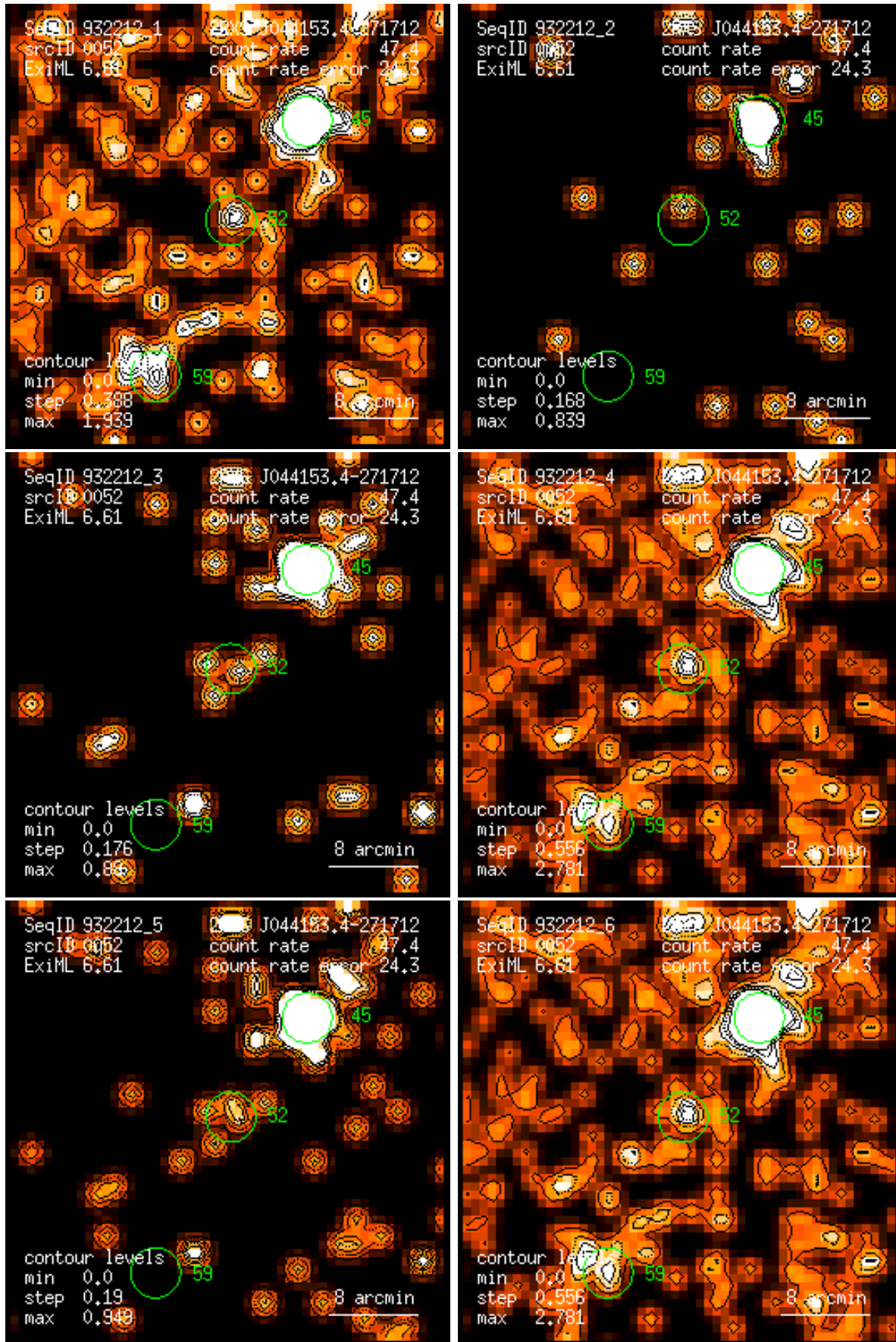
Figure 52: RASS 932212: detection 0052: band rate images, Gaussian filter: (1) PSPC channels 11 – 41, (2) 52 – 90, (3) 91 – 201, (4) 11 – 235, (5) 52 – 201, (6) 11 – 201. Broad band rates in counts/ks. Band rate contour levels in counts/ks/arcmin 2 .
