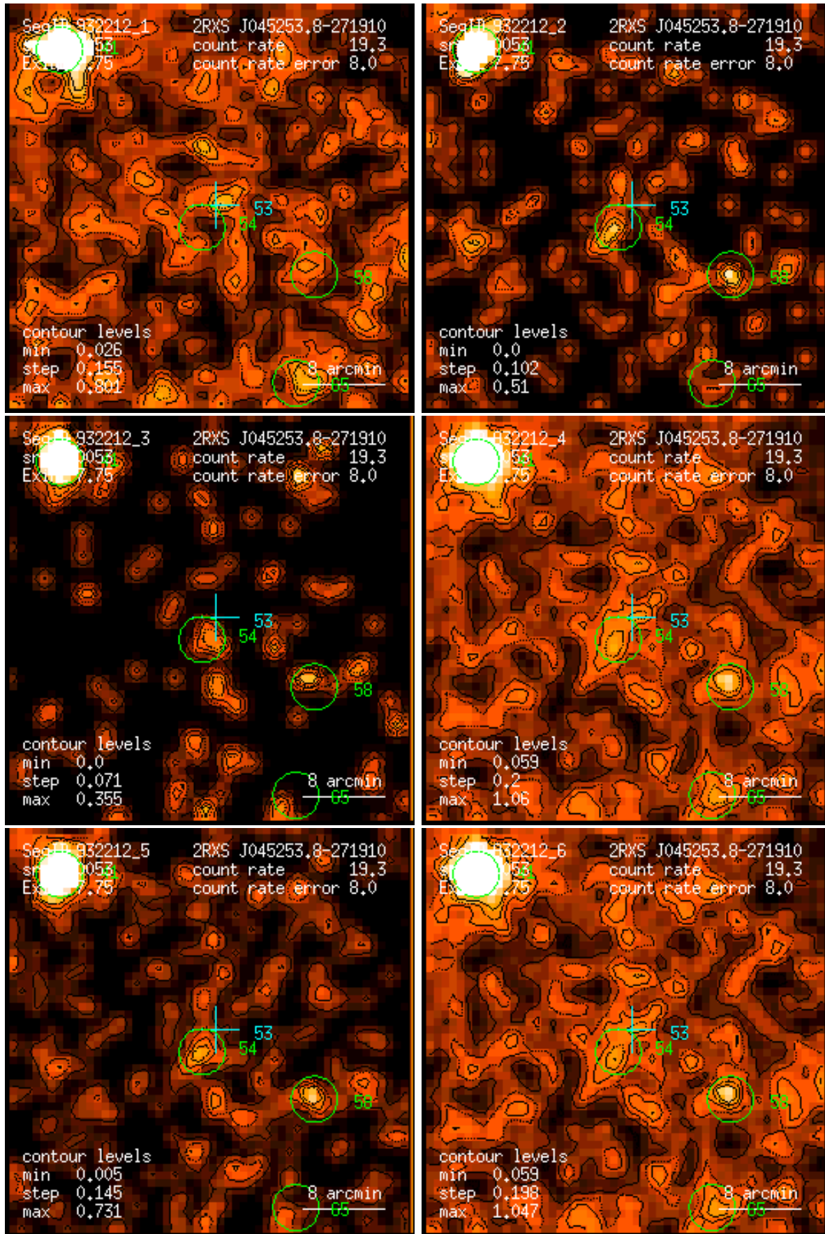
Figure 53: RASS 932212: detection 0053: band rate images, Gaussian filter: (1) PSPC channels 11 – 41, (2) 52 – 90, (3) 91 – 201, (4) 11 – 235, (5) 52 – 201, (6) 11 – 201. Broad band rates in counts/ks. Band rate contour levels in counts/ks/arcmin 2 .
