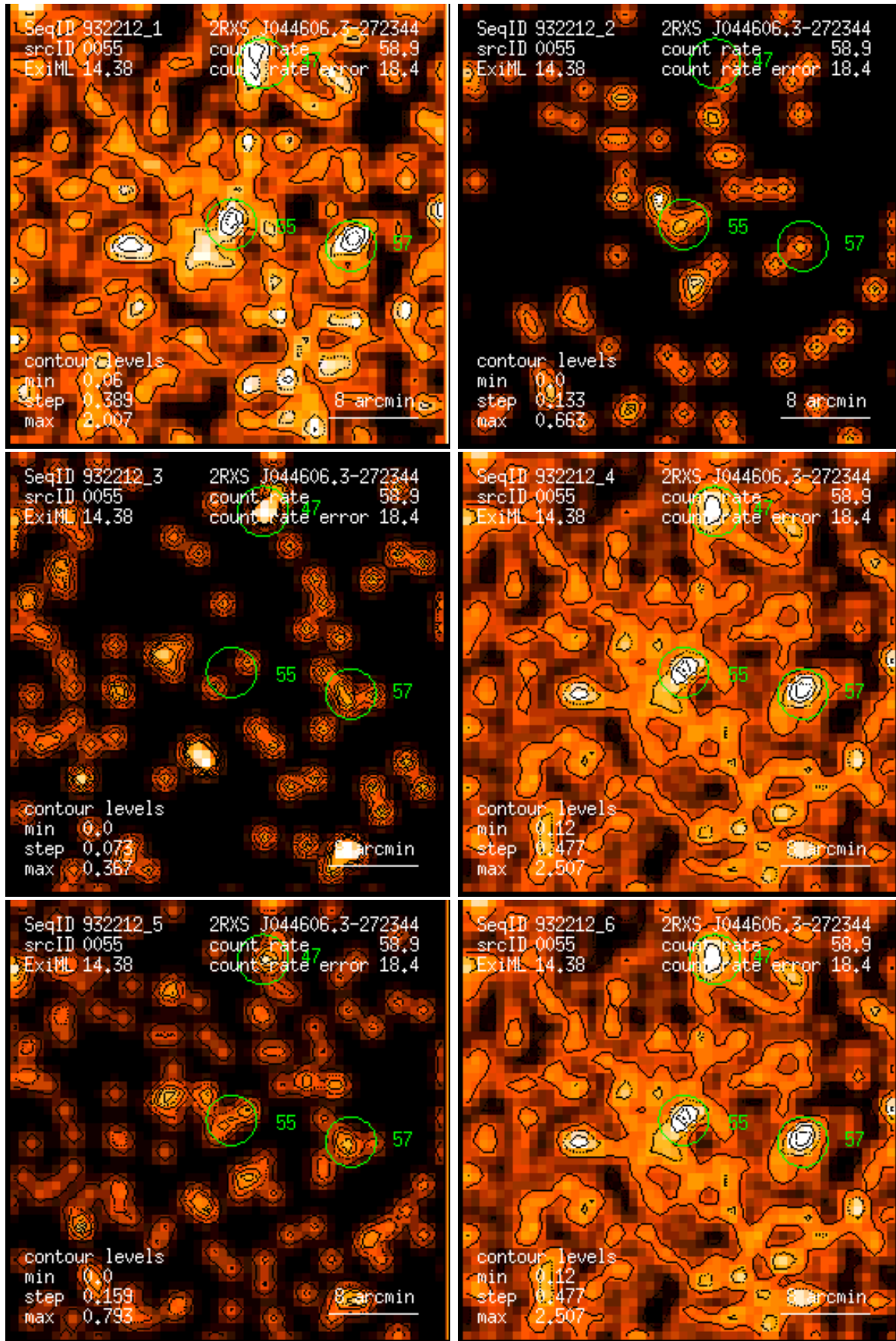
Figure 55: RASS 932212: detection 0055: band rate images, Gaussian filter: (1) PSPC channels 11 – 41, (2) 52 – 90, (3) 91 – 201, (4) 11 – 235, (5) 52 – 201, (6) 11 – 201. Broad band rates in counts/ks. Band rate contour levels in counts/ks/arcmin 2 .
