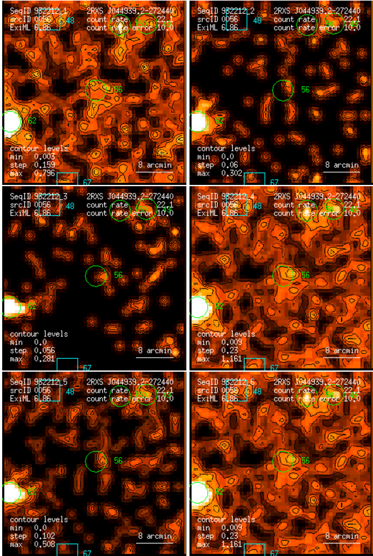
Figure 56: RASS 932212: detection 0056: band rate images, Gaussian filter: (1) PSPC channels 11 – 41, (2) 52 – 90, (3) 91 – 201, (4) 11 – 235, (5) 52 – 201, (6) 11 – 201. Broad band rates in counts/ks. Band rate contour levels in counts/ks/arcmin 2 .
