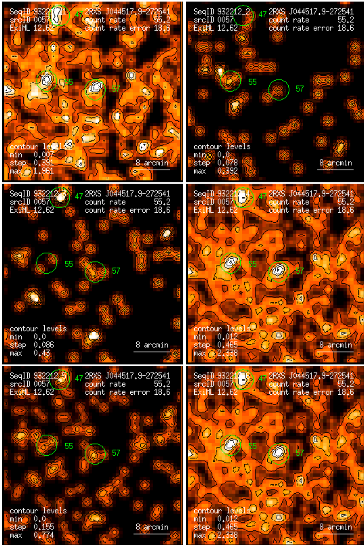
Figure 57: RASS 932212: detection 0057: band rate images, Gaussian filter: (1) PSPC channels 11 – 41, (2) 52 – 90, (3) 91 – 201, (4) 11 – 235, (5) 52 – 201, (6) 11 – 201. Broad band rates in counts/ks. Band rate contour levels in counts/ks/arcmin 2 .
